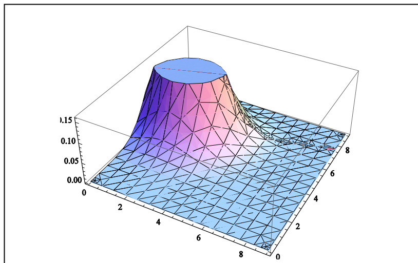
Figure 3-16 IF-THEN Rule by Mamdini Gaussian Implication
