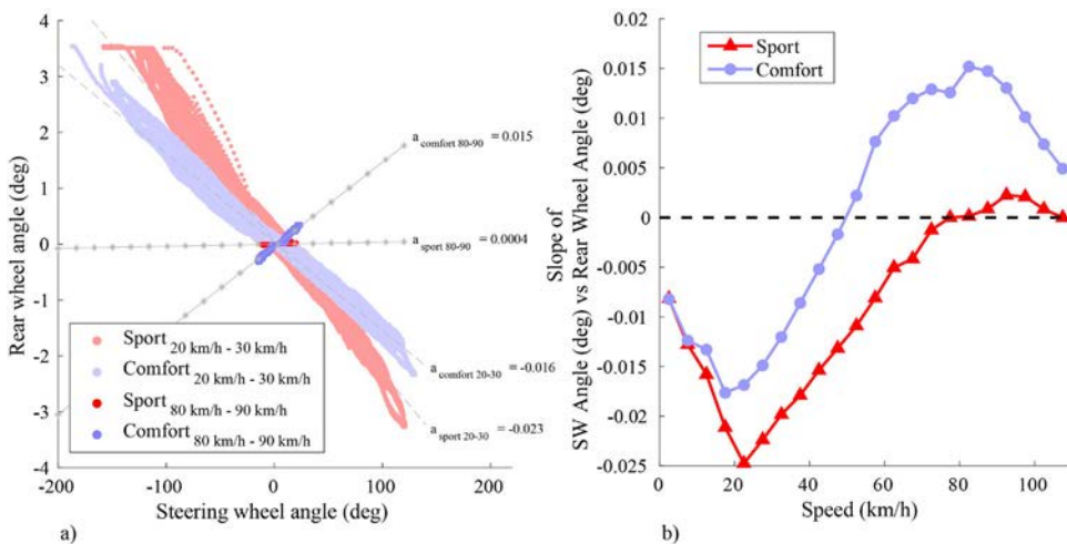
Figure 9. Rear-wheel angle as a function of steering wheel angle for the sport (red) and comfort mode (blue). (a) Steering wheel angle and rear wheel angle between 20 and 30 km/h (light) and 80 and 90 km/h (dark). (b) The slope of the linear regression between steering wheel angle and rear wheel angle per 5 km/h speed bin. Results are based on the combined route and the four repetitions combined.
