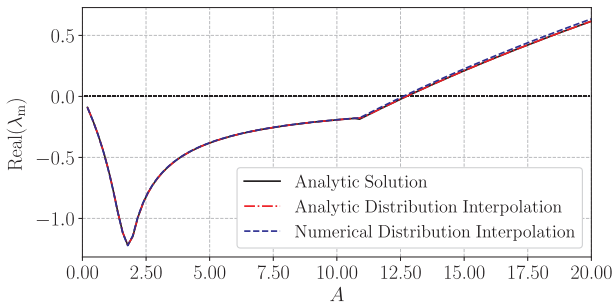
Fig. 4. Real part of the rightmost eigenvalues of (18) with K = 2 , a = 0.15 , b = 2 and z_m = 42 as a function of A .
