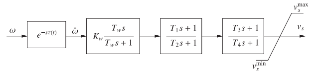
Fig. 6. Control scheme of Power System Stabilizer.
