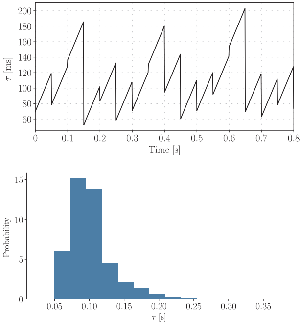
Fig. 7. WAMS Delay Model A: time-varying delay with analytic PDF.
