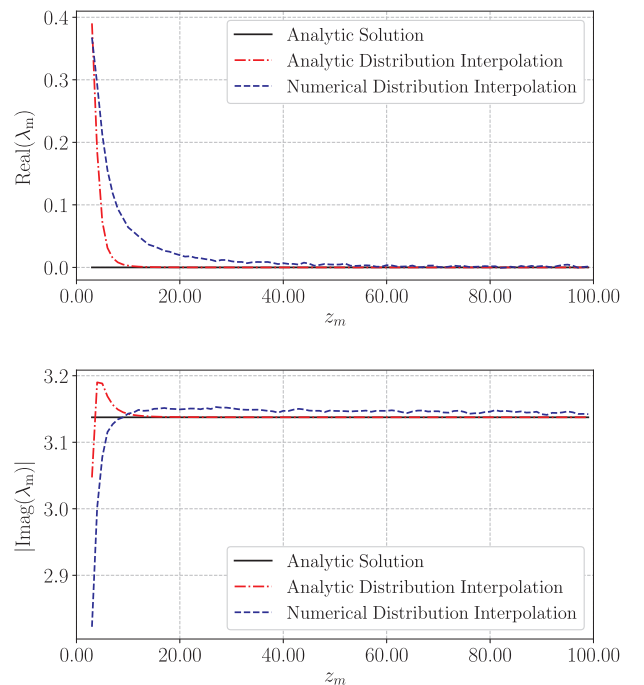
Fig. 3. Real part of the rightmost eigenvalues of (18) with A = 5, K = 2, a = 0.3187 and b = 2 as functions of z_m .
