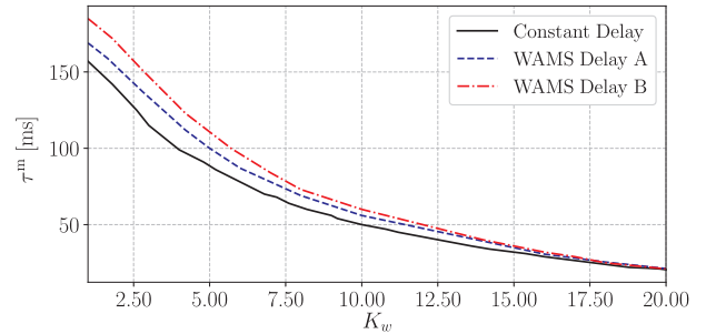
Fig. 9. Delay Margin of the IEEE 14-bus system as a function of K_w .
