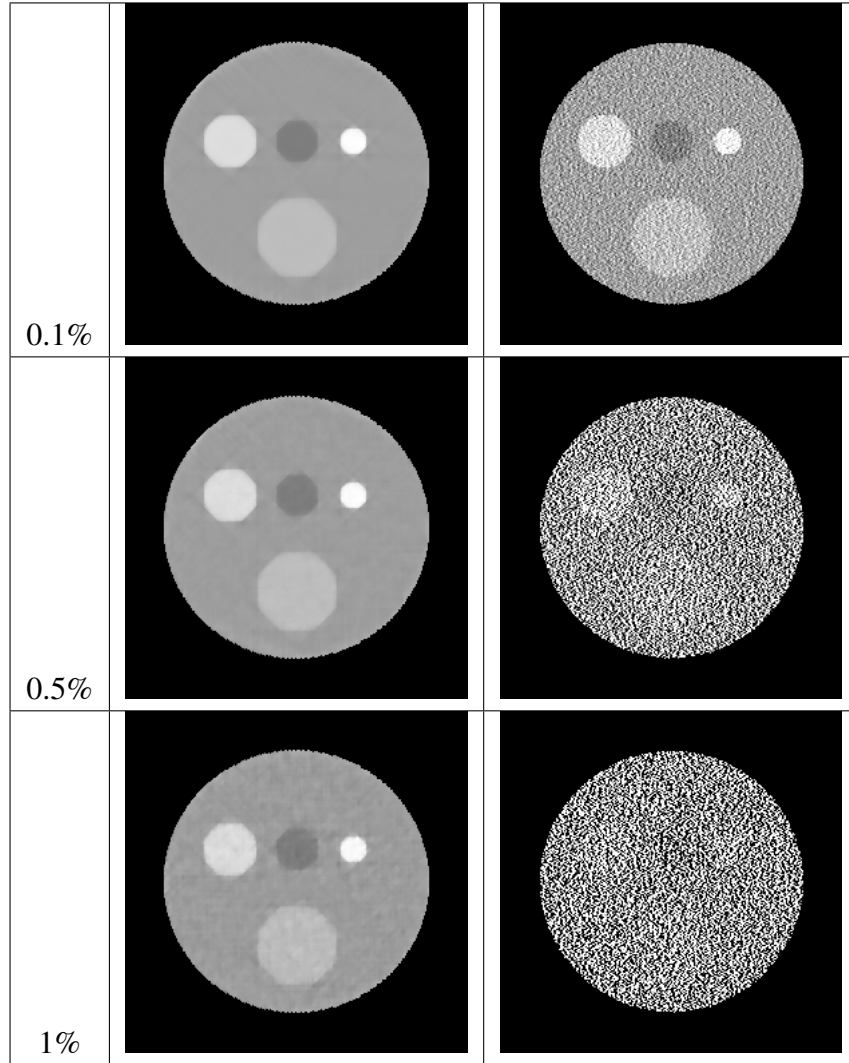
Figure 3.13: Reconstructions from four-detector data contaminated by noise of various levels, energy-independent attenuation. Left - iterative algorithm, right - inversion formula (3.11) with optimal C_j, j = 1, \dots, 4 (cf. (3.34)).
