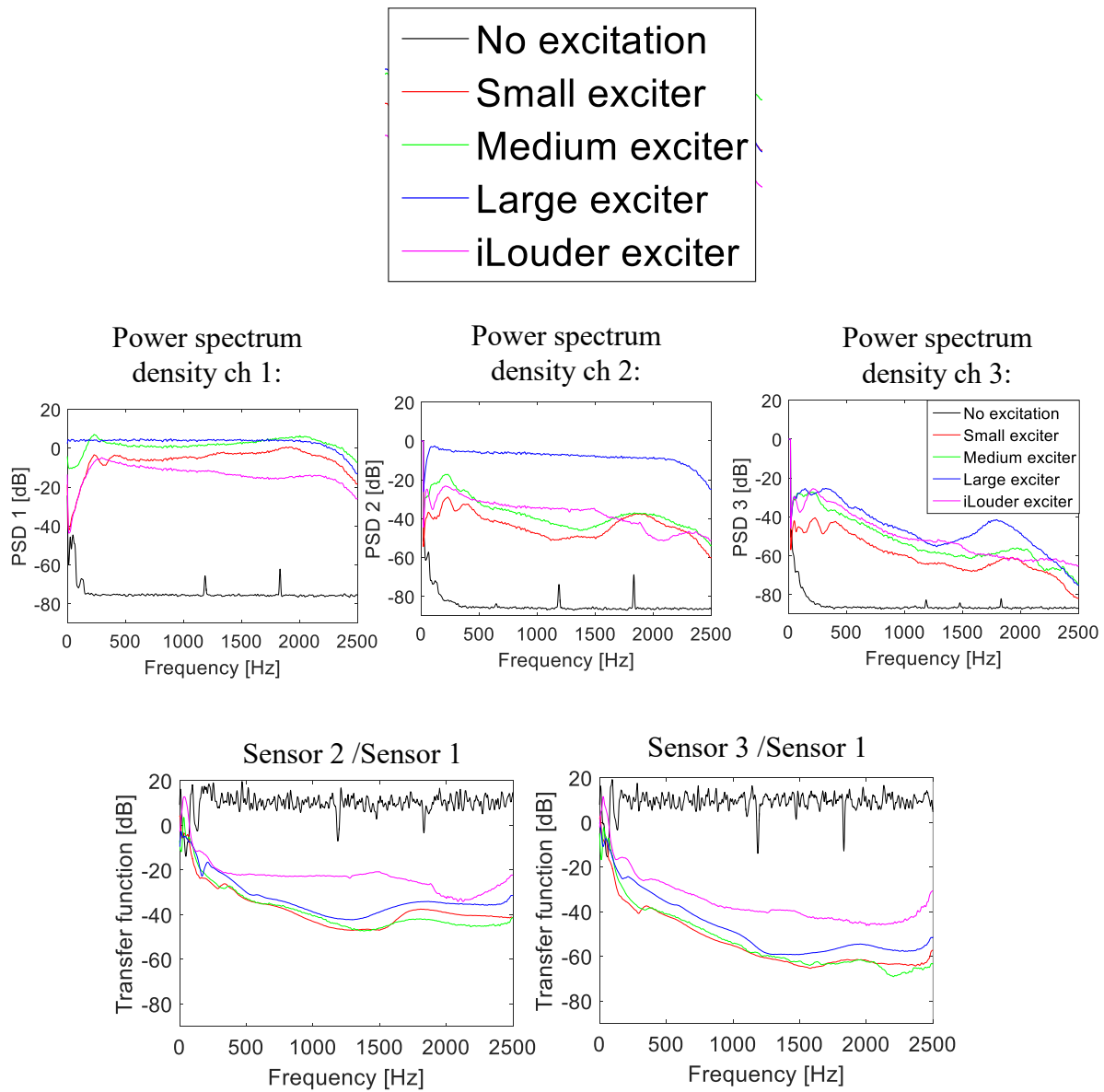
Figure 28: Power spectrum density for different exciter at excitation and measurement points. Transfer function between excitation and measurement points for different exciter.
