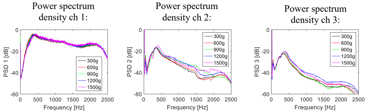
Figure 24: Effect of applied static load on iLouder exciter for human subject at excitation and measurement points PSD for sensor 1, sensor 2, and sensor 3.
