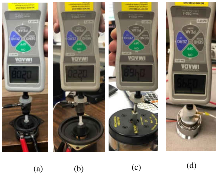
Figure 10: Experimental set up to study the effect of static load using the benchtop model of soft tissue on (a) small exciter, (b) medium exciter, (c) large exciter, and (d) iLoudr exciter
