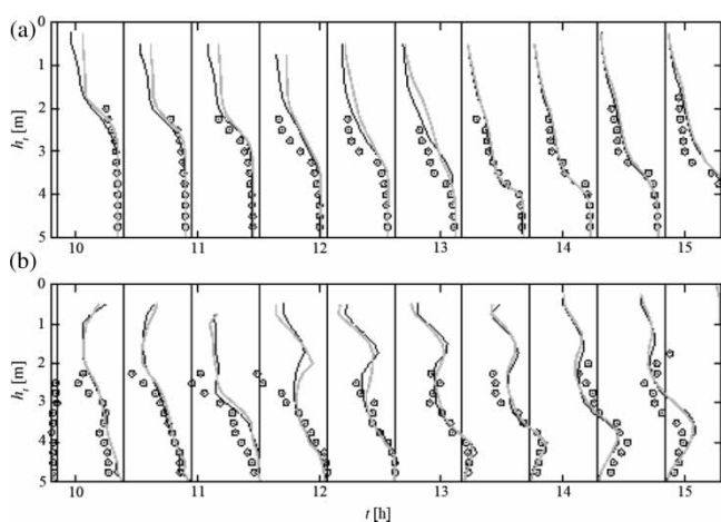
Figure 4 Stagger plot of field and simulated values of (a) salinity ( 1\text{ h} = 30\text{ psu} ), (b) longitudinal velocity ( 1\text{ h} = 1\text{ m s}^{-1} ) for \Delta z = 12.5\text{ cm} . (open circle) field data, (black solid line) ELCOM with YIG closure, (grey solid line) ELCOM with LIHF closure, (dashed grey line) zeros
