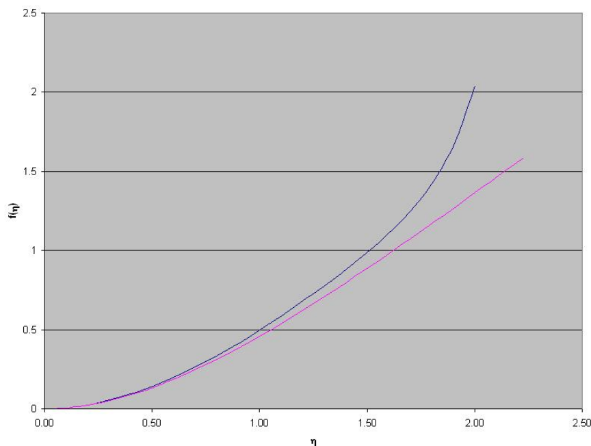
Figure 3.1: Solution Comparison to Numerical Solution
