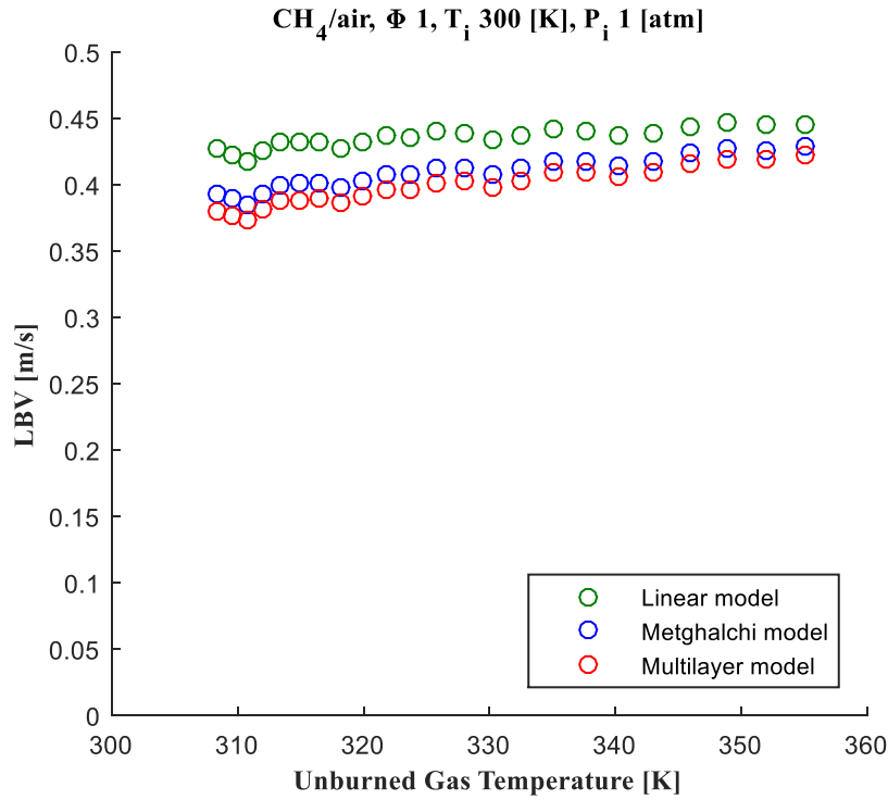
Figure 3.6. Laminar burning velocity comparison for stoichiometric CH 4 /air mixture at an initial temperature 300 [K] and initial pressure of 1 [atm].
