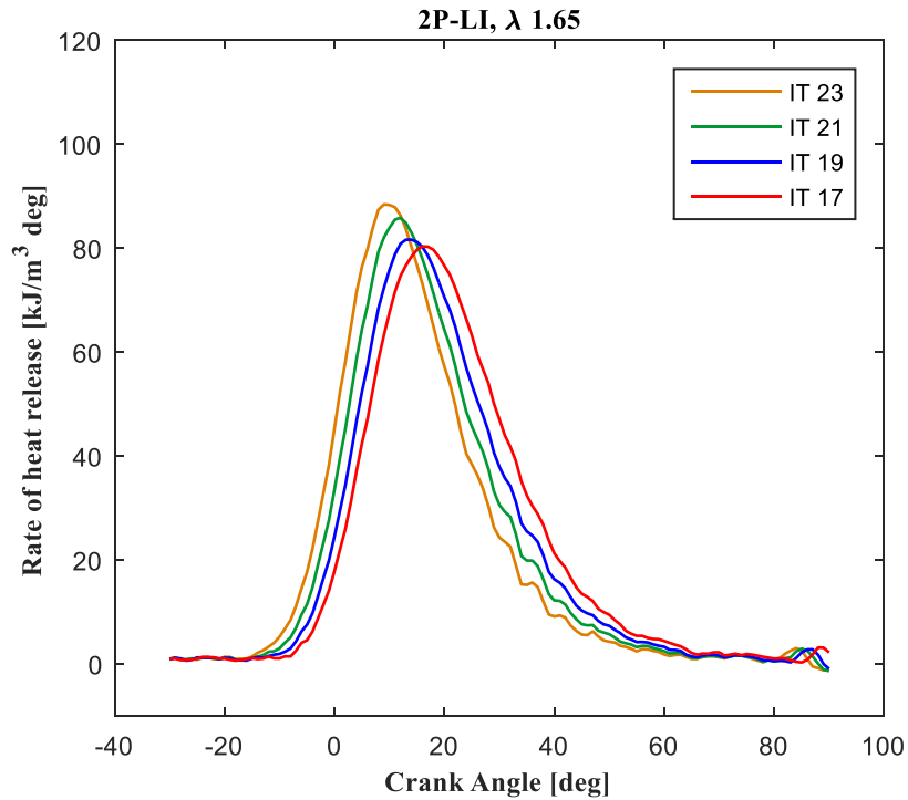
Figure C20. Rate of heat release of a natural gas reciprocating engine operated with laser ignition at fixed air to fuel ratios \lambda = 1.65 and several ignition timings in CA BTDC.
