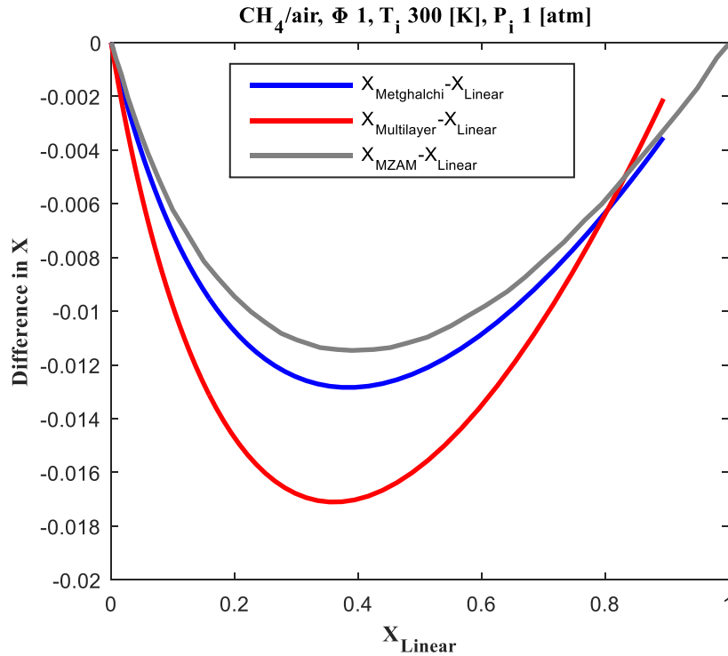
Figure 3.3. Models comparison based on the difference of mass fraction burned for stoichiometric CH 4 /air mixture at an initial temperature 300 [K] and initial pressure of 1 [atm].
