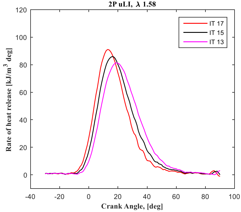
Figure C19. Rate of heat release of a natural gas reciprocating engine operated with laser ignition at fixed air to fuel ratios \lambda = 1.58 and several ignition timings in CA BTDC.
