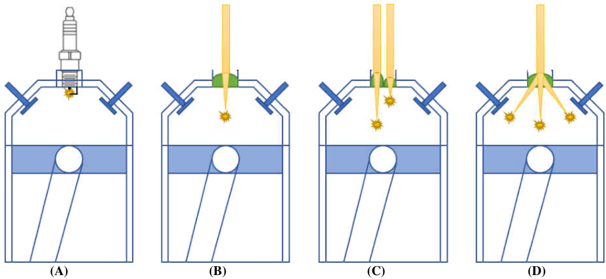
Figure 2.1. Schematics of reciprocating engines ignited by (A) a spark plug, (B) a laser ignitor with a single pulse, (C) two laser ignitors with two focal lengths (D) a laser ignitor with multi-point ignition.
