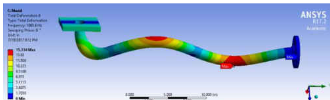
Figure 37 The 6th Mode for FPA, 1 Inch Diameter, SS, 24 Inches Long
