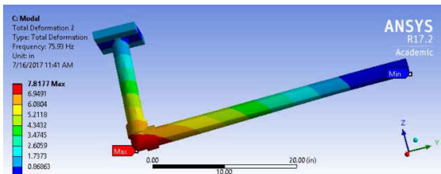
Figure 252 The 2nd Mode for SWPA, 2 Inch Diameter, CS, 36 Inches Long
