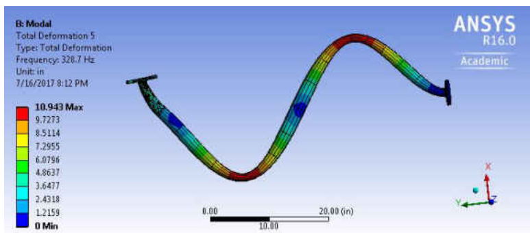
Figure 117 The 5th Mode for FPA, 1 Inch Diameter, CS, 48 Inches Long
