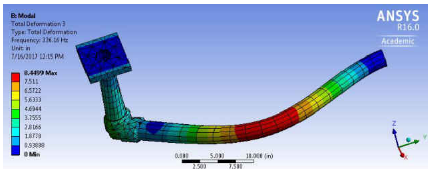
Figure 277 The 3rd Mode for SWPA, 2 Inch Diameter, SS, 36 Inches Long
