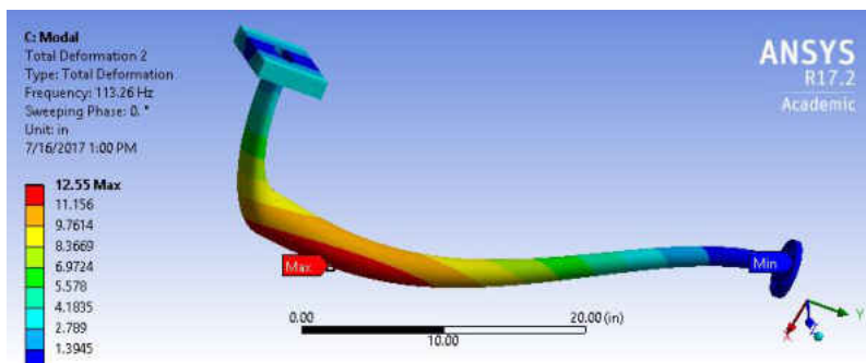
Figure 132 The 2nd Mode for FPA, 1 Inch Diameter, SS, 36 Inches Long
