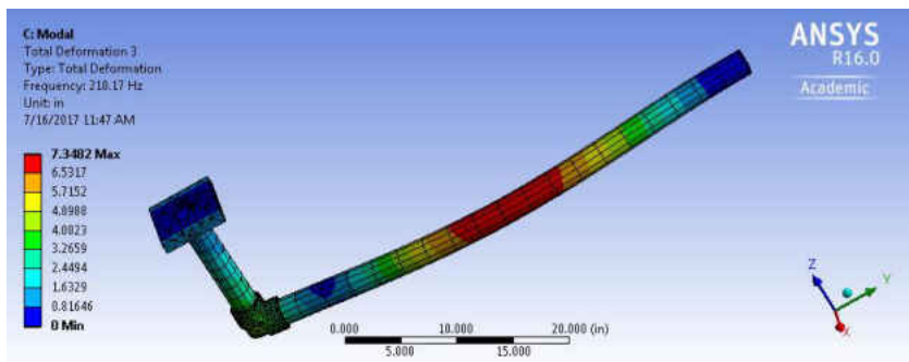
Figure 259 The 3rd Mode for SWPA, 2 Inch Diameter, CS, 48 Inches Long
