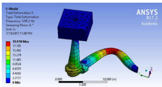
Figure 70 The 5th Mode for SWPA, 1 Inch Diameter, CS, 12 Inches Long
