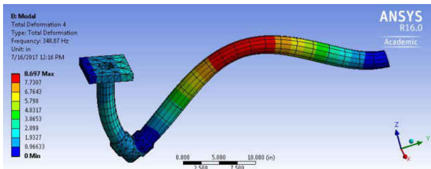
Figure 278 The 4th Mode for SWPA, 2 Inch Diameter, SS, 36 Inches Long
