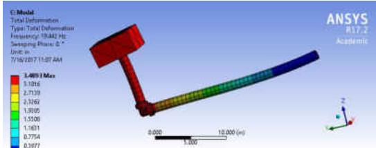
Figure 72 The 1st Mode for SWPA, 1 Inch Diameter, CS, 24 Inches Long
