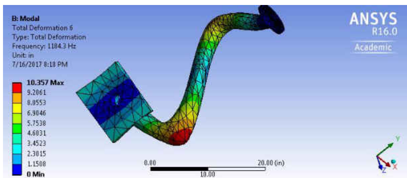
Figure 178 The 6th Mode for FPA, 2 Inch Diameter, SS, 24 Inches Long
