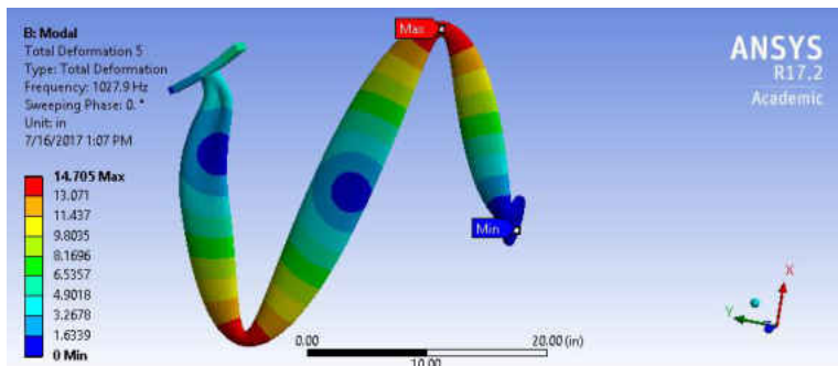
Figure 105 The 5th Mode for FPA, 1 Inch Diameter, CS, 24 Inches Long
