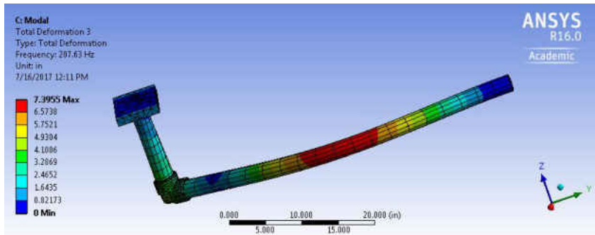
Figure 283 The 3rd Mode for SWPA, 2 Inch Diameter, SS, 48 Inches Long
