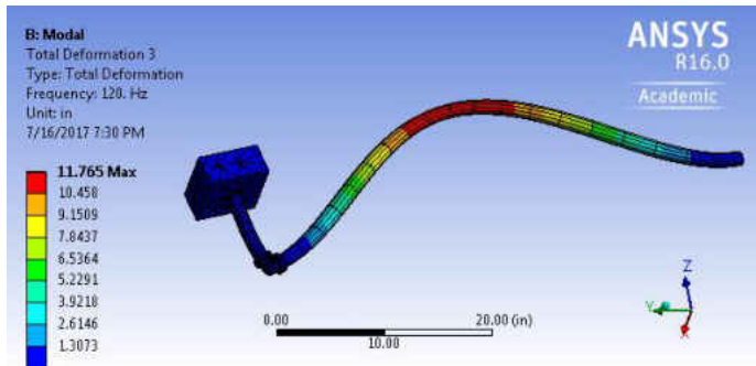
Figure 211 The 3rd Mode for SWPA, 1 Inch Diameter, CS, 48 Inches Long
