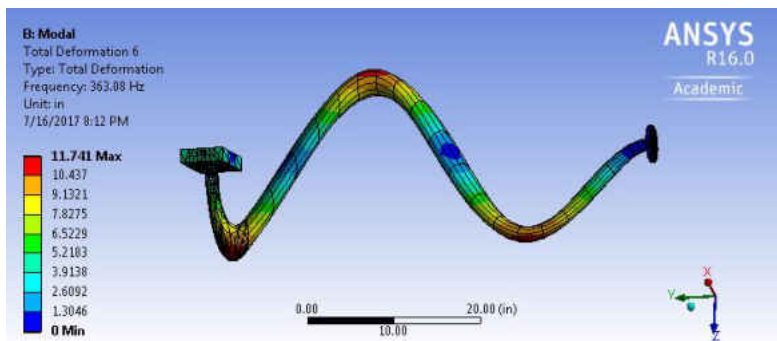
Figure 118 The 6th Mode for FPA, 1 Inch Diameter, CS, 48 Inches Long
