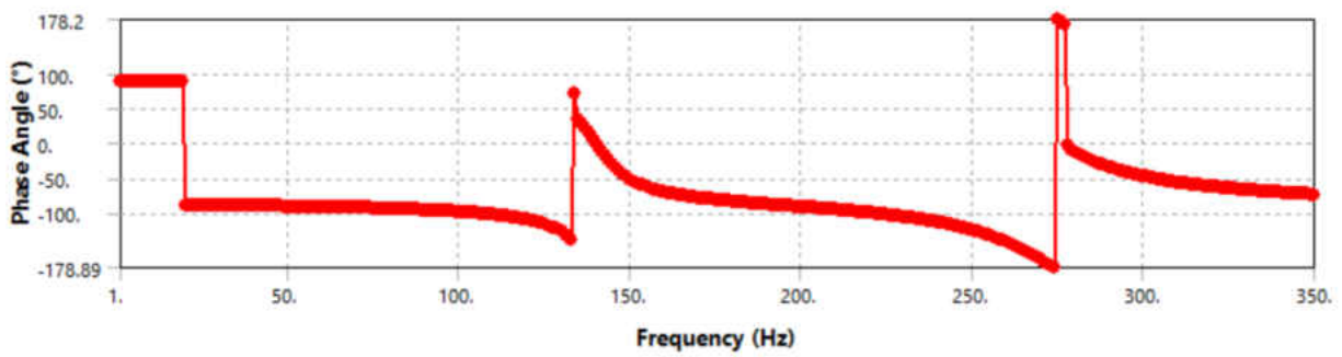
Figure 80 Phase Angle and Amplitude of SWPA, CS, 1" Diameter, 24" Long
