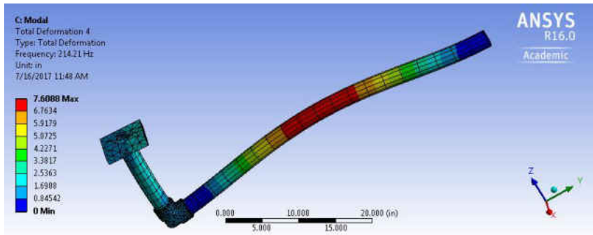
Figure 260 The 4th Mode for SWPA, 2 Inch Diameter, CS, 48 Inches Long
