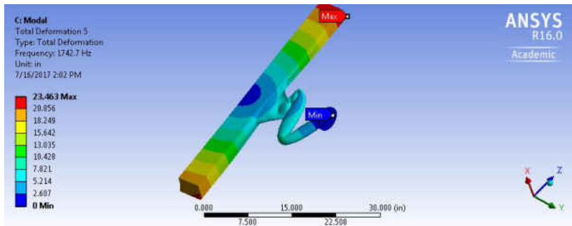
Figure 99 The 5th Mode for FPA, 1 Inch Diameter, CS, 12 Inches Long
