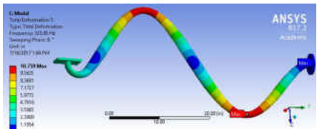
Figure 33 The 5th Mode for FPA, 1 Inch Diameter, SS, 48 Inches Long
