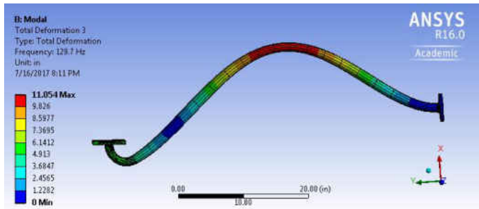
Figure 115 The 3rd Mode for FPA, 1 Inch Diameter, CS, 48 Inches Long
