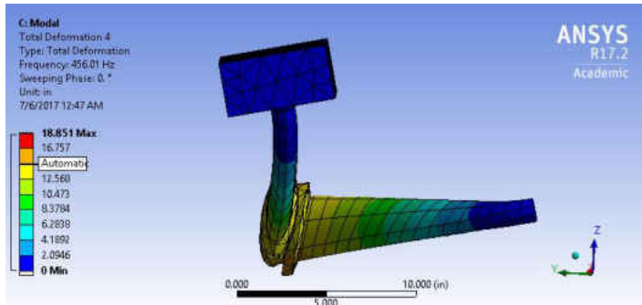
Figure 22 The 4th Mode for CS 12 Inch Pipe, at 456.01 Hz
