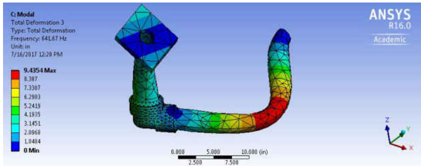
Figure 271 The 3rd Mode for SWPA, 2 Inch Diameter, SS, 24 Inches Long
