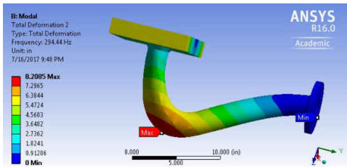
Figure 168 The 2nd Mode for FPA, 2 Inch Diameter, SS, 12 Inches Long
