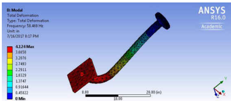
Figure 173 The 1st Mode for FPA, 2 Inch Diameter, SS, 24 Inches Long
