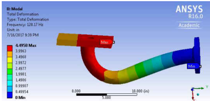
Figure 167 The 1st Mode for FPA, 2 Inch Diameter, SS, 12 Inches Long
