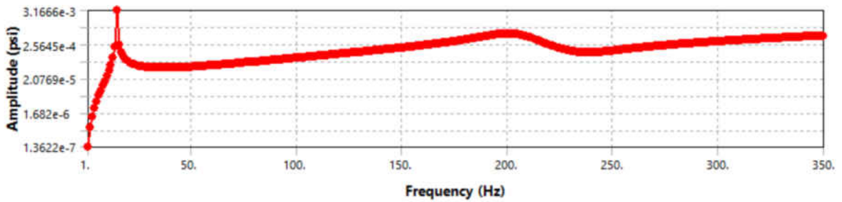
Figure 84 Phase Angle and Amplitude of SWPA, SS, 1" Diameter, 24" Long
