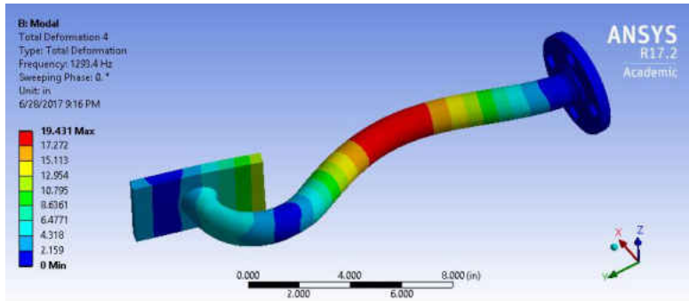
Figure 11 The 3rd Mode for CS 24 Inch Pipe, at 1293.4 Hz
