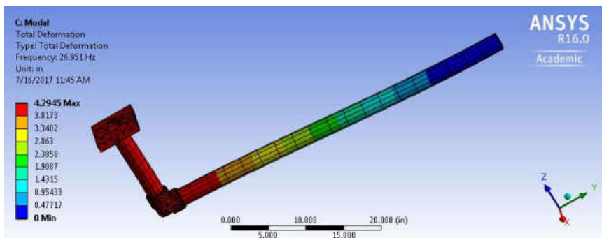
Figure 257 The 1st Mode for SWPA, 2 Inch Diameter, CS, 48 Inches Long
