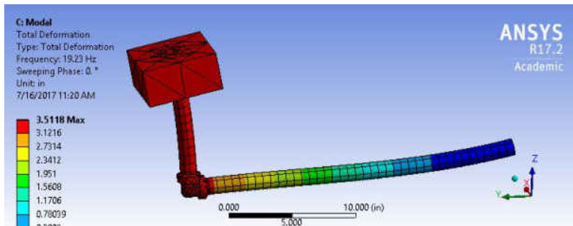
Figure 221 The 1st Mode for SWPA, 1 Inch Diameter, SS, 24 Inches Long
