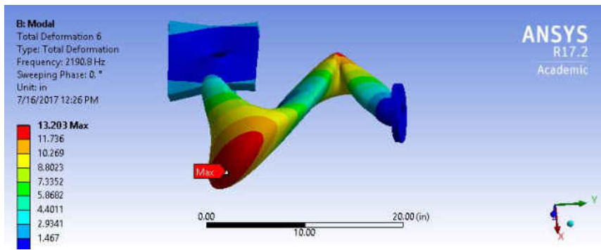
Figure 148 The 6th Mode for FPA, 2 Inch Diameter, CS, 12 Inches Long
