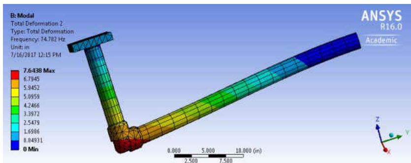
Figure 276 The 2nd Mode for SWPA, 2 Inch Diameter, SS, 36 Inches Long
