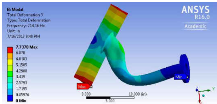
Figure 169 The 3rd Mode for FPA, 2 Inch Diameter, SS, 12 Inches Long
