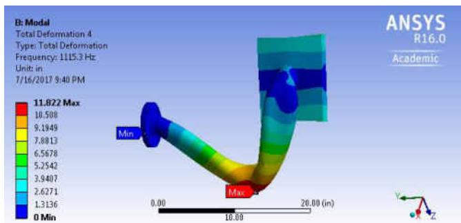
Figure 170 The 4th Mode for FPA, 2 Inch Diameter, SS, 12 Inches Long
