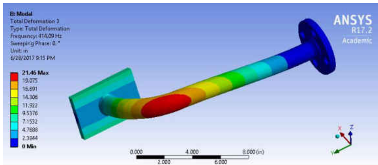
Figure 10 The 2nd Mode for CS 24 Inch Pipe, at 414.09Hz
