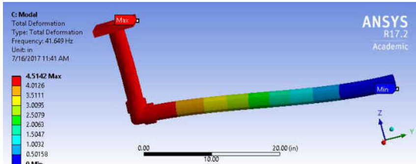
Figure 251 The 1st Mode for SWPA, 2 Inch Diameter, CS, 36 Inches Long
