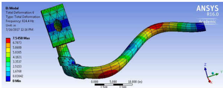
Figure 280 The 6th Mode for SWPA, 2 Inch Diameter, SS, 36 Inches Long
