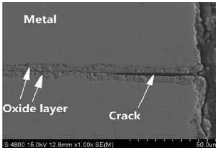
Figure 2-6: Oxide spikes formed at the surface from compressive dwells.[10]
