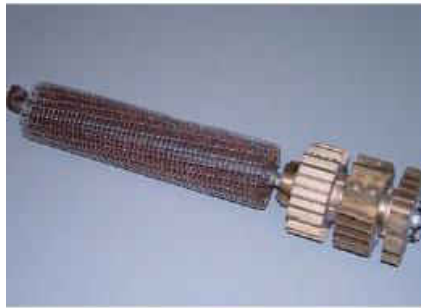
Figure 17) a) Detailed view inside the heat exchanger elements b) heat exchanger c) ceramic tube d) steel housing
