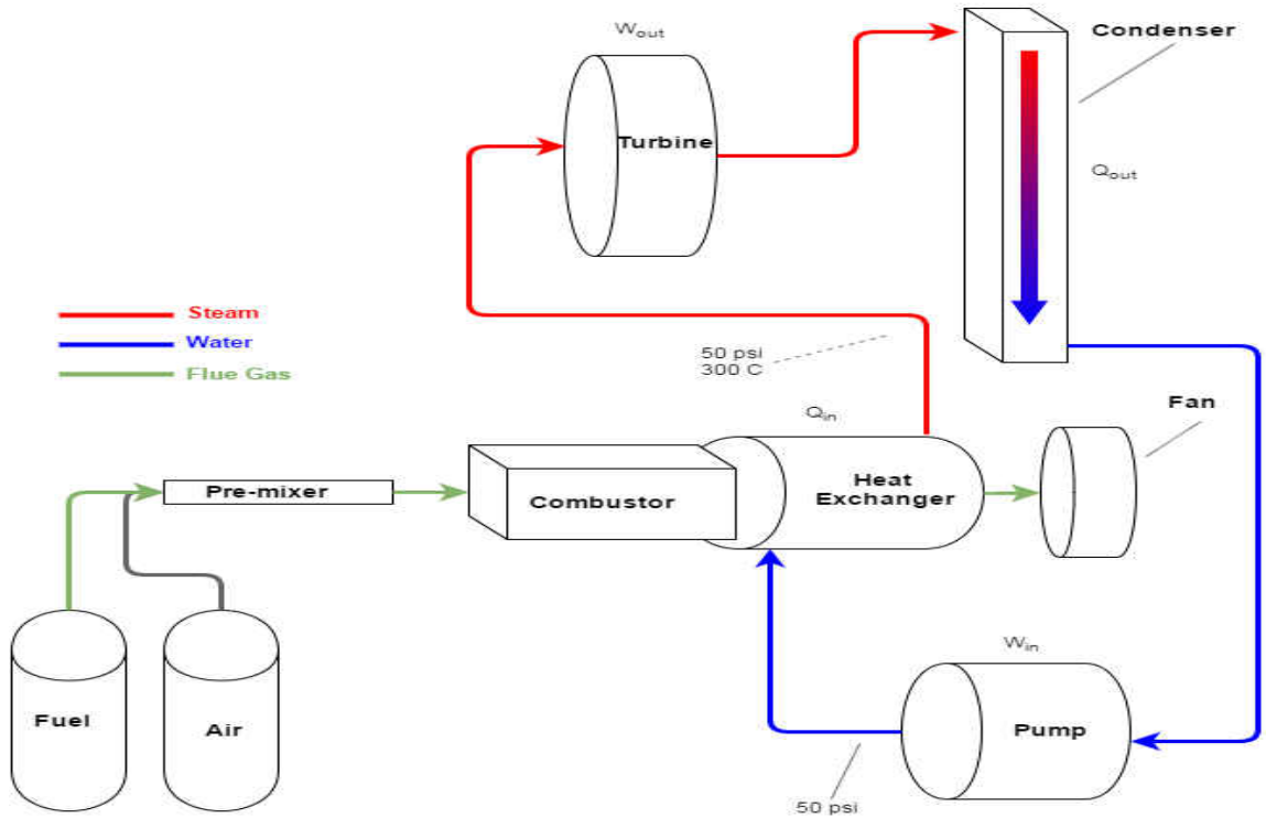
Figure 32) Process Schematic
