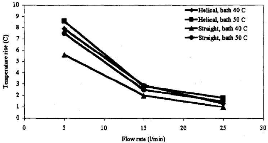
Figure 27) Temperature vs Flow rate for different temperatures of the helical bath for both helical and straight tubes for helical coil and straight pipe
