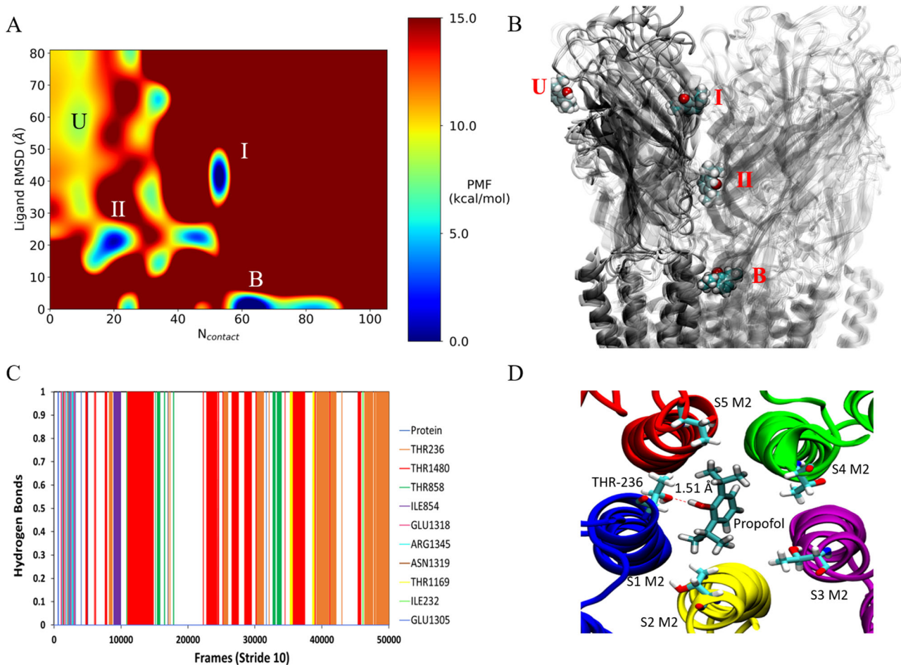
Figure 4. GaMD simulations captured pore binding of propofol: (A) 2D ( N_{\text{contact}} , propofol RMSD) PMF calculated by reweighting the 500 ns GaMD simulation. (B) Pathway of propofol diffusion into the M2 helix pore in all three GaMD simulations. (C) Hydrogen-bonds formed between propofol and the GLIC, where bonds formed after 10000 steps are in the pore. Protein refers to short lived hydrogen-bonds formed on the protein exterior. Data combined from all three replicates. (D) Final frame snapshot showing propofol hydrogen-bonding to Thr-236 in S1.
