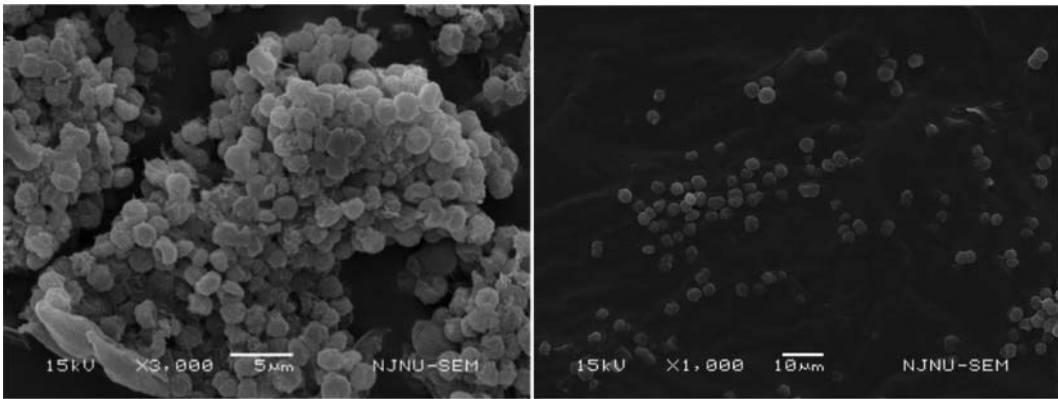
Figure 4. Electron micrographs of colonial (left) and single (right) Microcystis aeruginosa in different zoom multiples.
