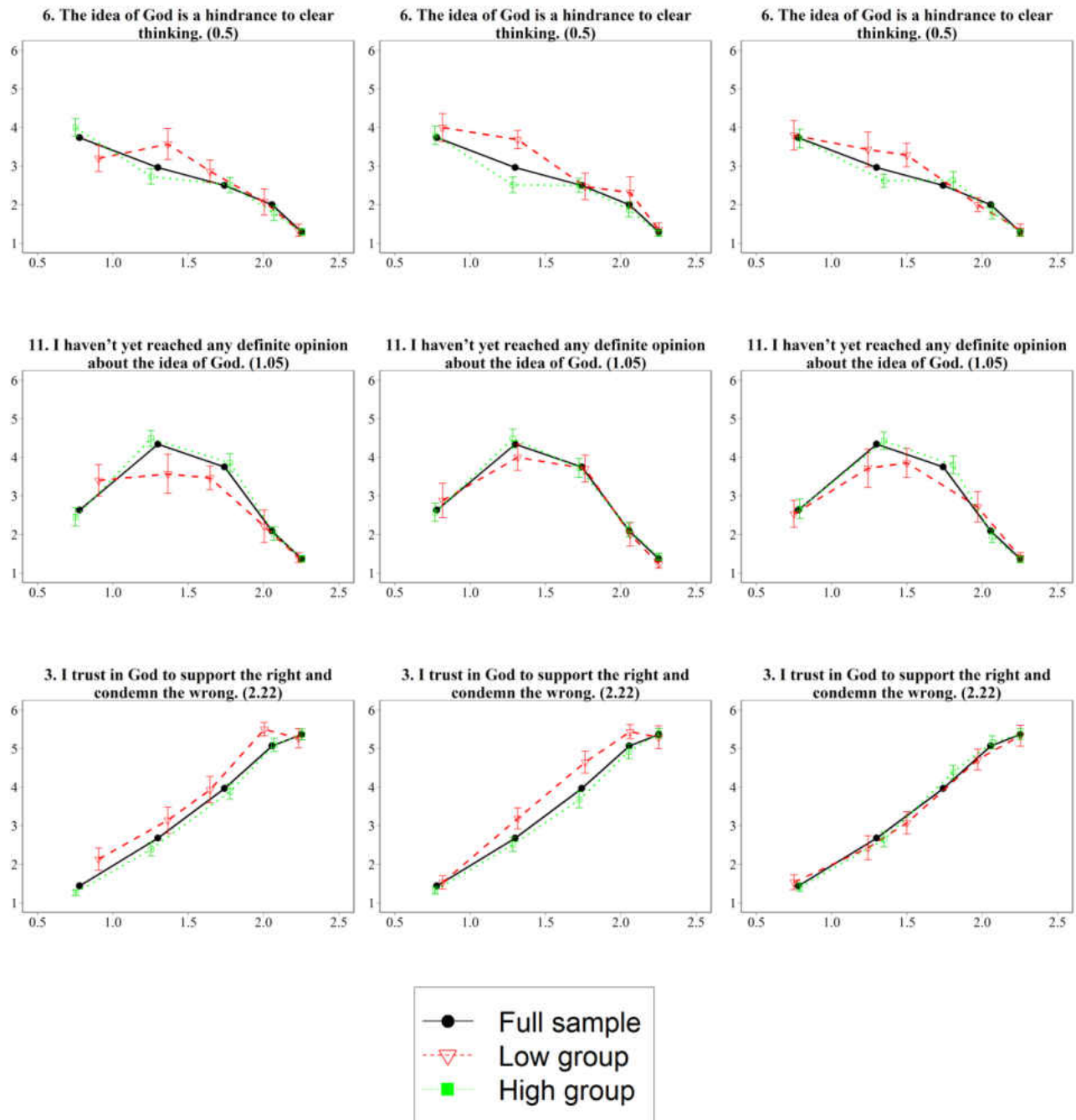
Figure 15. Moderated Item Characteristic Curves – God
