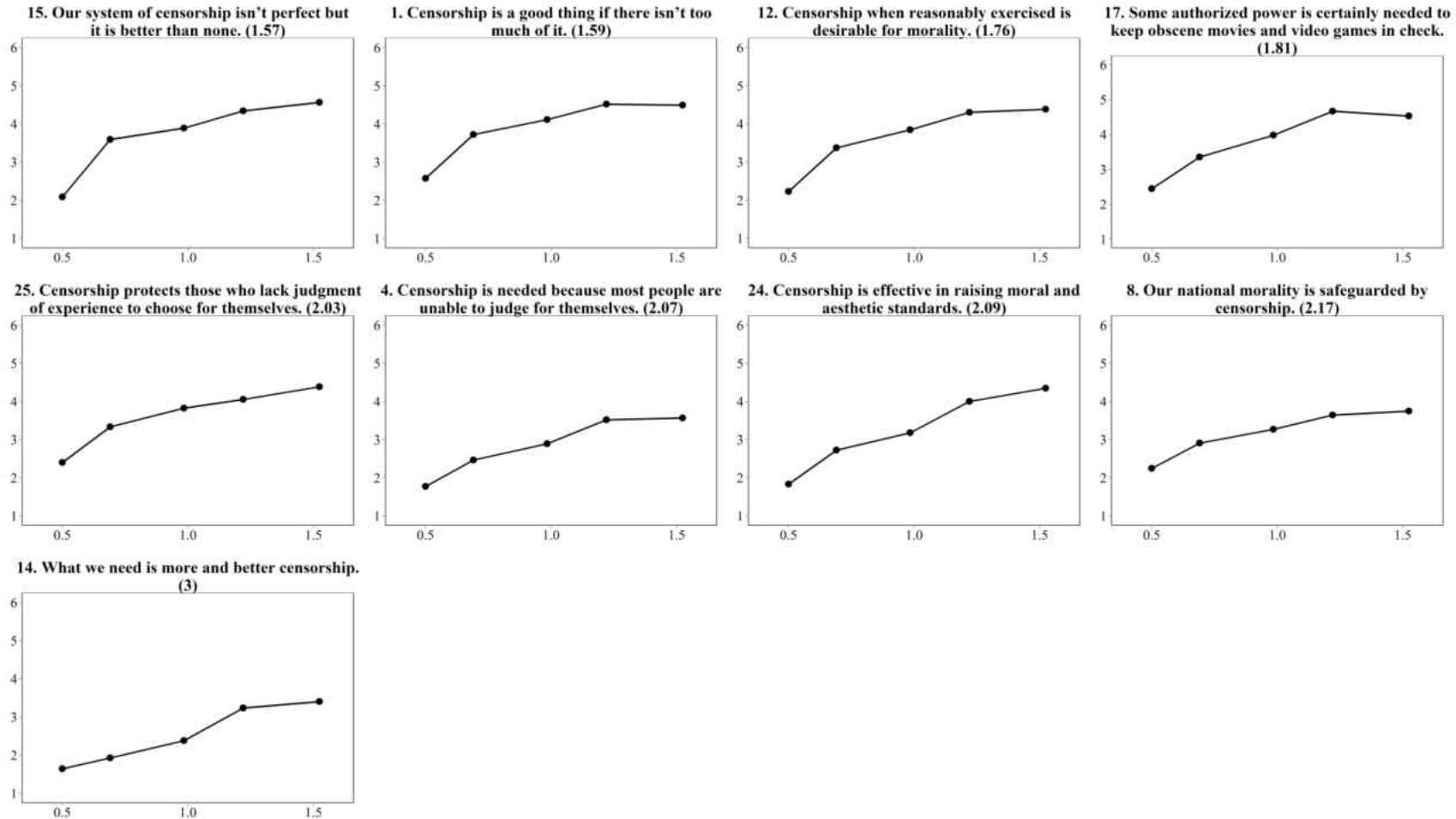
Figure 12. Item Characteristic Curves – Censorship
