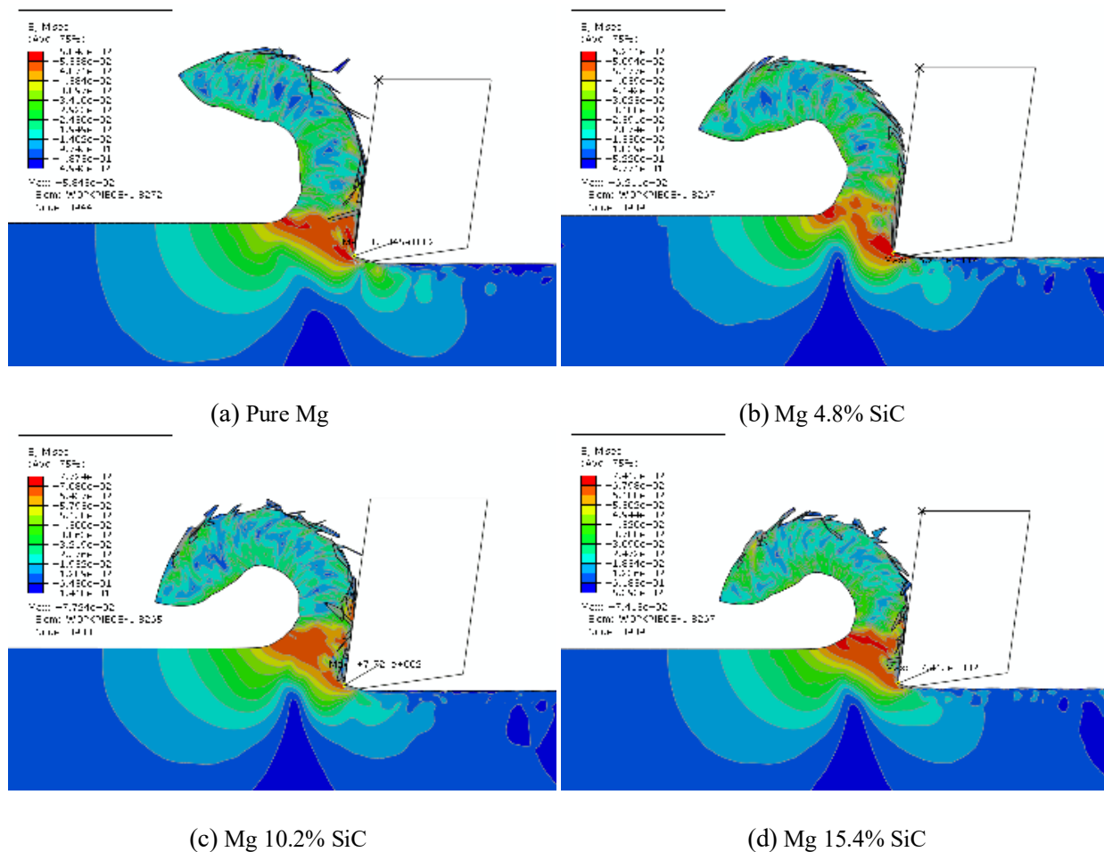
Figure 6.4: Von Mises stress distribution of the (a) Pure Magnesium and (b) ~ (d) Mg-MMCs with different weight fractions of SiC nanoparticles
