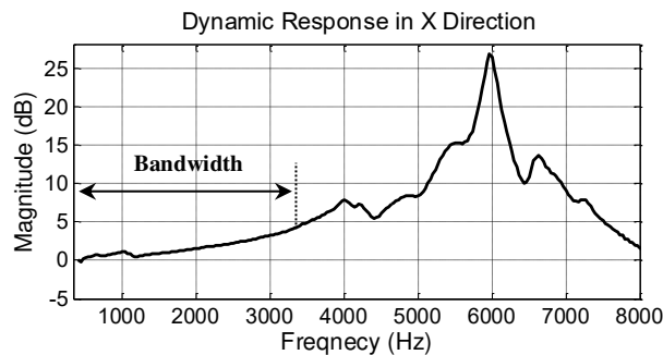
Figure 4.9: Dynamic response in the X direction of the dynamometer from the impact hammer test
