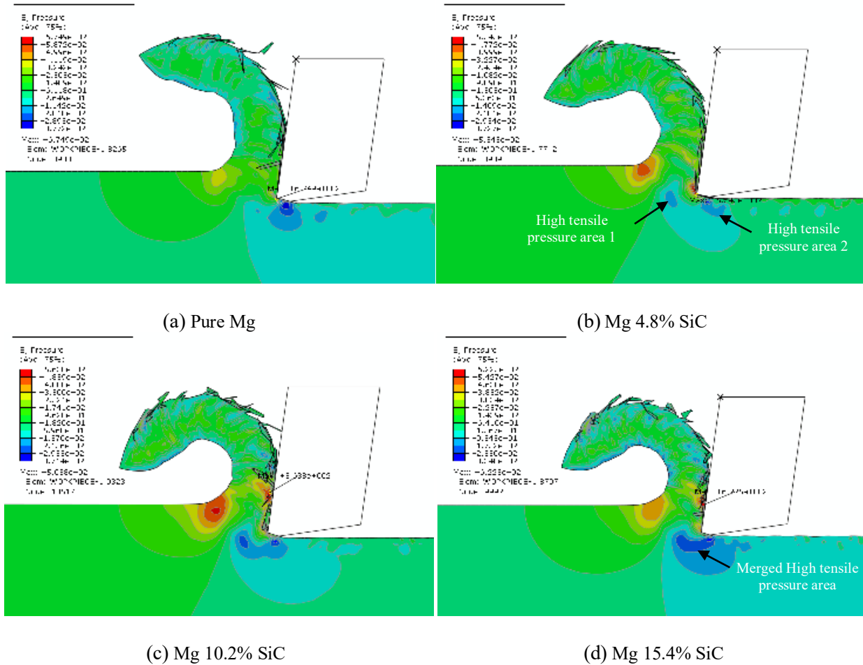
Figure 6.6: Pressure stress distribution of the (a) Pure Magnesium and (b) ~ (d) Mg-MMCs with different weight fractions of SiC nanoparticles
