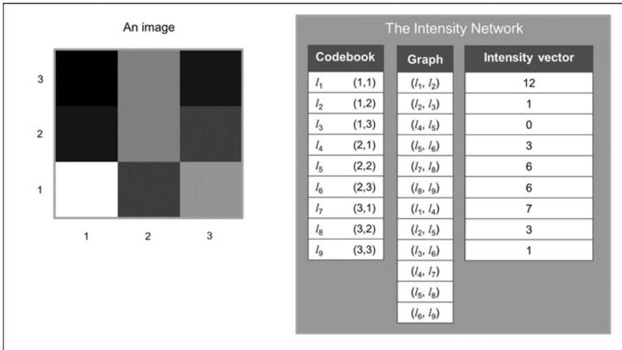
Figure 1. Right: a typical IN. Left: the image it refers to. The codebook encodes the location of the pixels (note the coordinates in this example are indexed from top to bottom, then left to right). The graph structure encodes the neighborhood relationships between the pixels; the couples (l_i, l_j) are ordered so that i < j . The intensity vector encodes the values of the pixels.
