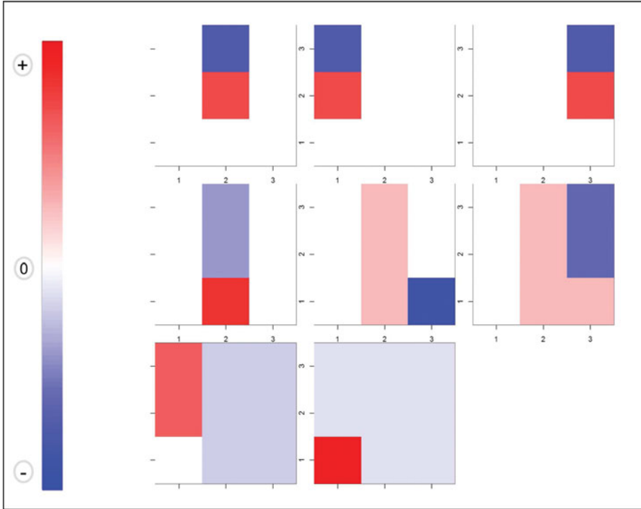
Figure 5. Basis functions \{\Psi_k\}_{k=p-1\dots 1} for the image of Figure 1, obtained in the order of their construction, for rank k = p - 1 (top left), \dots , k = 2 (bottom left), k = 1 (bottom right), with p (the number of pixels) being equal to 9. The remaining basis function \Psi_0 is constant. The basis functions are orthonormal and, except for \Psi_0 , reflect level changes between contiguous zones in the image.
