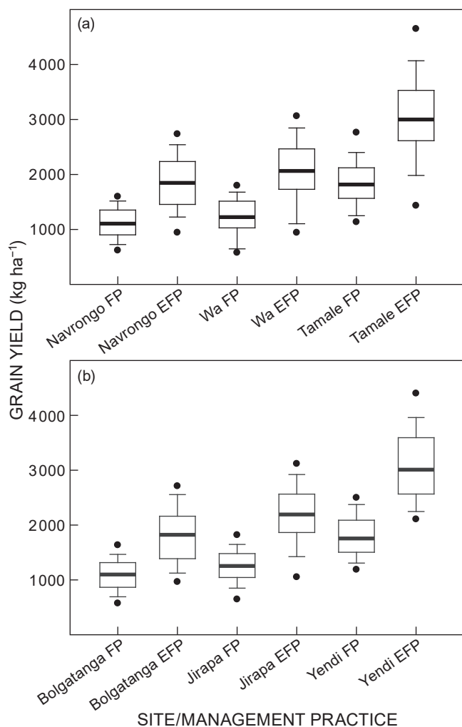
Figure 5: Comparison of simulated maize yield of farmer current farmer practice (CFP) and enhanced farmer practice (EFP) across all six sites. Each box indicates the 25th, 50th and 75th percentiles, error bars indicate the 10th and 90th percentiles, and solid circles represent the 5th and 95th percentiles
