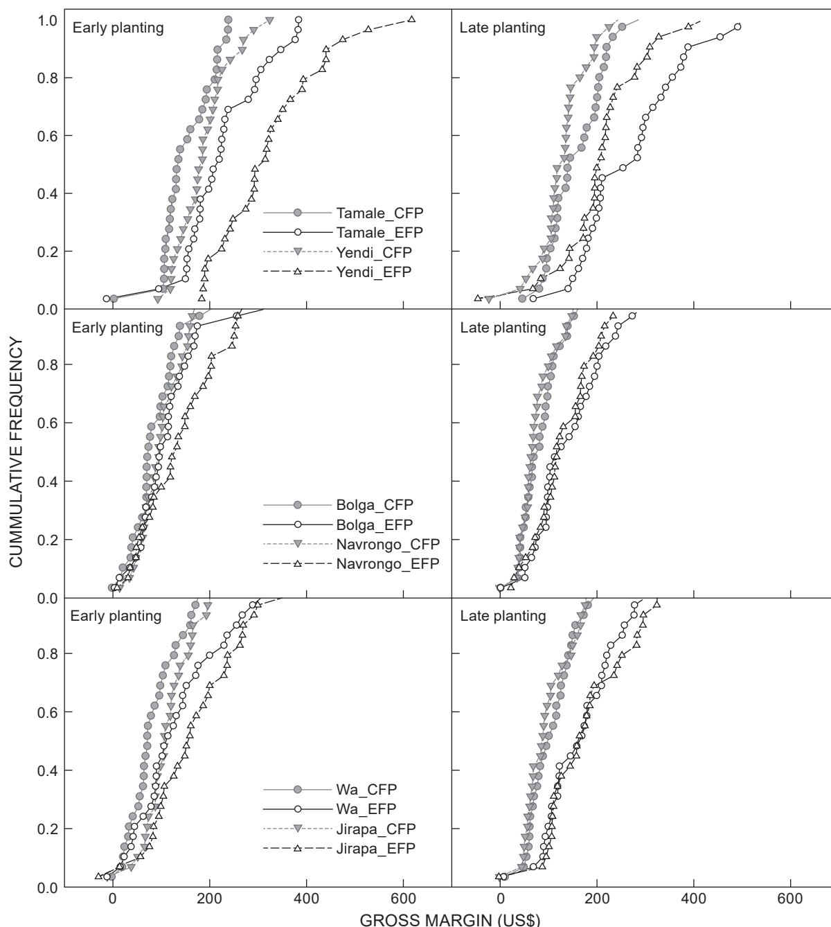
Figure 6: Comparison of estimated gross margins obtainable from current farmer practice (CFP) and enhanced farmer practice (EFP) across all six sites. CFP and EFP had inputs of 30 kg N ha -1 + 1 000 kg ha -1 manure and 60 kg N ha -1 + 2 000 kg ha -1 manure, respectively
