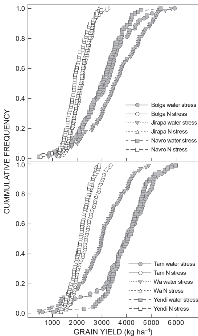
Figure 4: Comparison of simulated yields under water-limited (rain-fed, no nitrogen [N] stress) and N-limited (30 kg N ha -1 and no water stress) across the six sites over 30 years and three sowing windows. Tam = Tamale, Bolga = Bolgatanga, Navro = Navrongo
