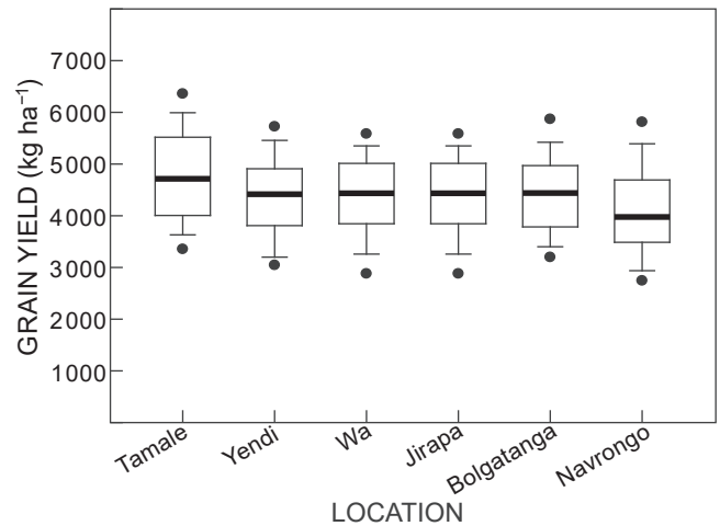
Figure 2: Variability in simulated potential yield of maize in six locations in northern Ghana. Each box indicates the 25th, 50th and 75th percentiles, error bars indicate the 10th and 90th percentiles, and solid circles represents the 5th and 95th percentiles
