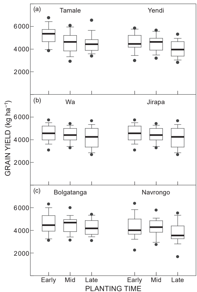
Figure 3: Variation of simulated potential yields within sites for different planting windows for the (a) Northern, (b) Upper West and (c) Upper East regions of Ghana. Each box indicates the 25th, 50th and 75th percentiles, error bars indicate the 10th and 90th percentiles and solid circles represent the 5th and 95th percentiles
