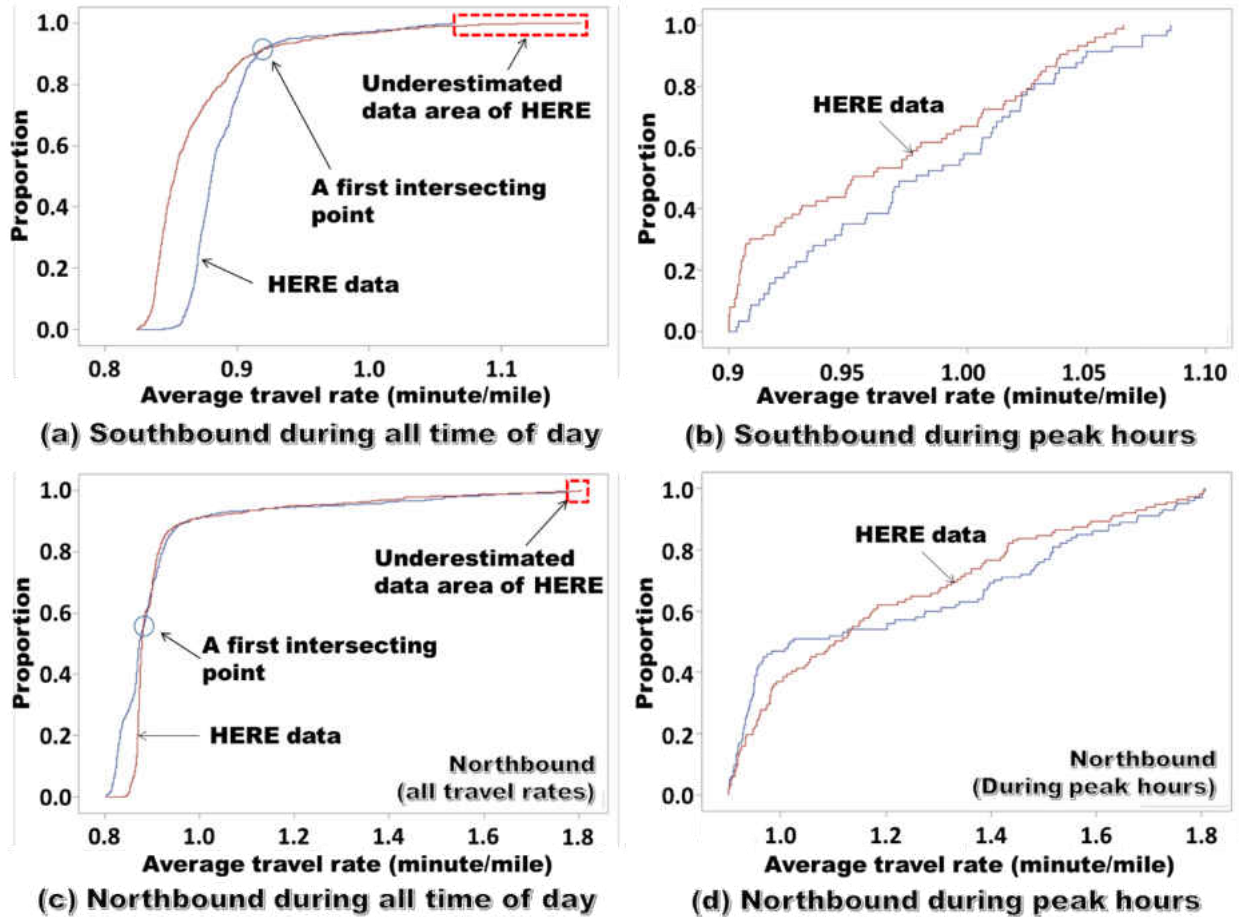
Figure 12. Empirical Cumulative Distributions (ECD) of average travel rate for time of day in 5-minute increments
