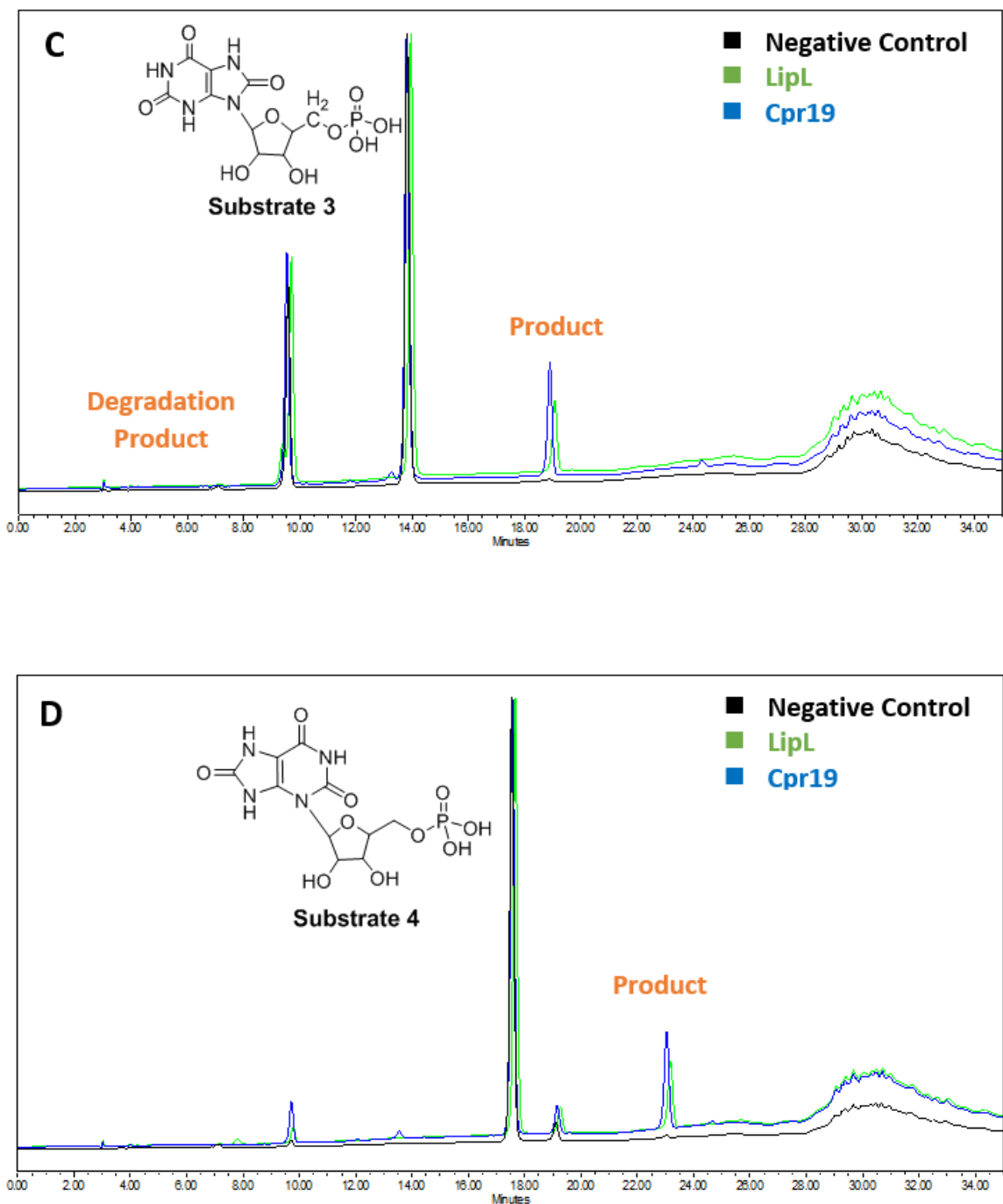
Figure 3.3.6.1. HPLC analyses of reactions catalyzed by Cpr19 and LipL when tested with substrate analogs XMP (A), S2 (B), S3 (C) and S4 (D). In all four chromatograms negative controls are shown in black , while reactions catalyzed by LipL and Cpr19 are indicated in green and blue respectively. In all four sets of reactions, the major peaks represent the respective substrate peaks as labeled, and the product peaks (indicated in orange in each set of reactions) were collected for further identification.
