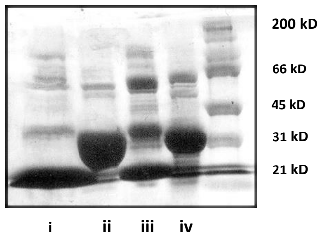
Figure 2.5.2.1. SDS-PAGE analysis of purified proteins (i) His 6 - phosphoriboisomerase or His 6 -EcRpiA (expected 22.8 kD), (ii) His 6 -Cpr19 (expected 31.7 kD), (iii) His 6 -uracil phosphopribosyl transferase or His 6 -EcUpp (expected 22.5 kD) and (iv) His 6 -5-phosphoribosyl-1-pyrophosphate synthetase or His 6 - StPRPPsynthase (expected 34 kD).
