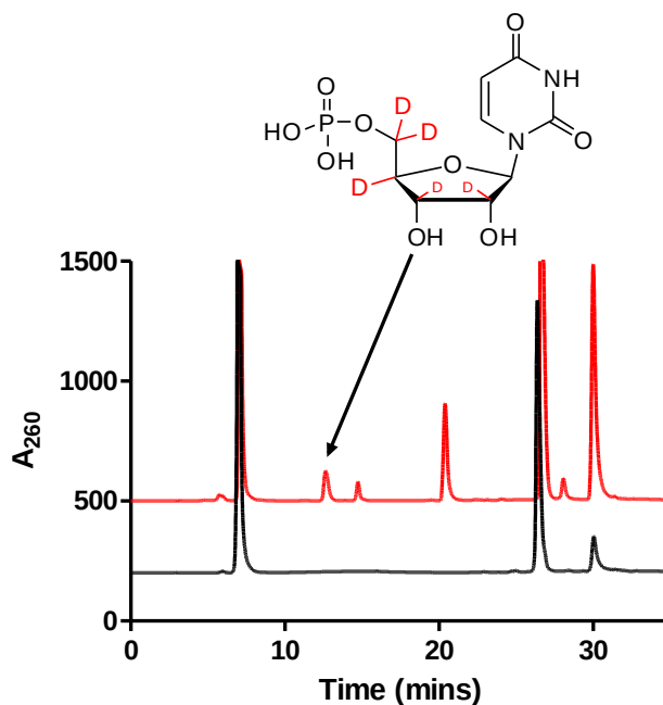
Figure 2.5.2.2. HPLC trace for the one-pot reaction. The pawthay is engineered from a combination of reactions adopted from the glycolytic and pentose phosphate pathways, and from nucleotide metabolism. The observed peak at t = 12 min corresponds to the
