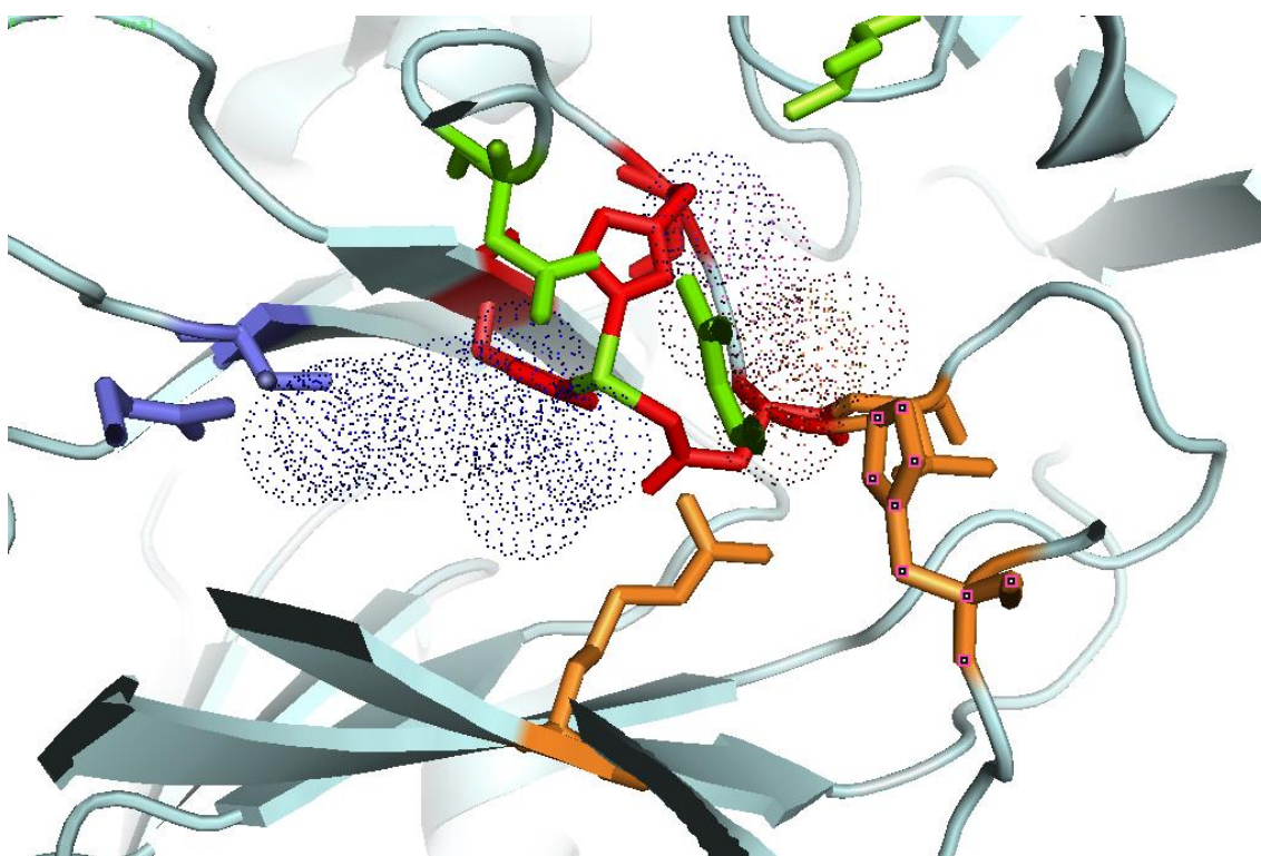
Figure 3.1.4. Catalytic pocket of TauD. Stereodiagram of TauD showing the protein ligands around the Fe(II) center. Shown here are the residues that form the facial triad (His 99, Asp 101, His 255) ( red ), alongside the other amino acid residues (Thr 126, Arg 266 in blue ) involved in stabilizing \alpha -KG (depicted in dots). The residues interacting with the amine end of primary substrate taurine are Tyr 73, Asn 95 and Ser 158 ( green ) while those involved in interacting with the sulfonate moiety are Arg 270, His 70 and the N-H backbone of Val 102 ( orange ).
