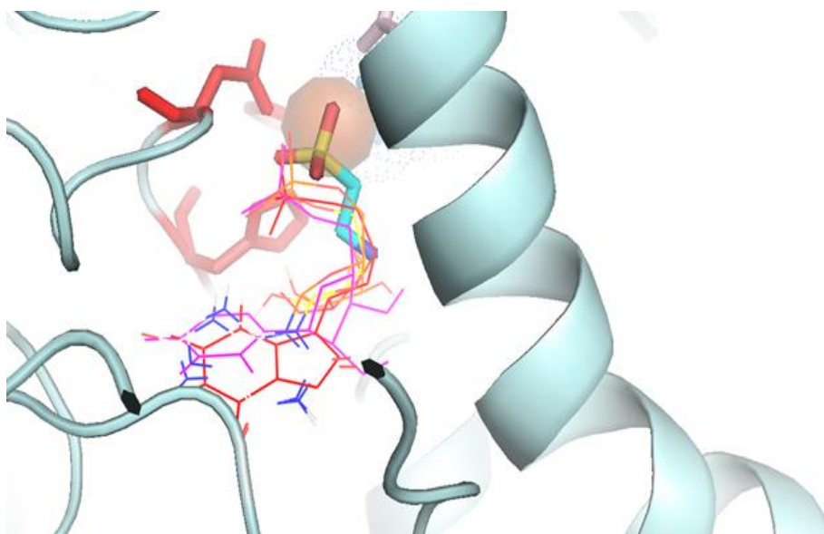
Figure 3.3.8.6. Docking all four substrate analogs into Cpr19 model. All four substrate analogs (XMP, S2, S3 and S4) are docked to overlap primary substrate UMP (shown in pink ), docked onto the active site. The predicted Cpr19 model can accommodate these relatively larger substrate analogs in a proposed cavity adjacent to the position of the taurine amine in TauD.
