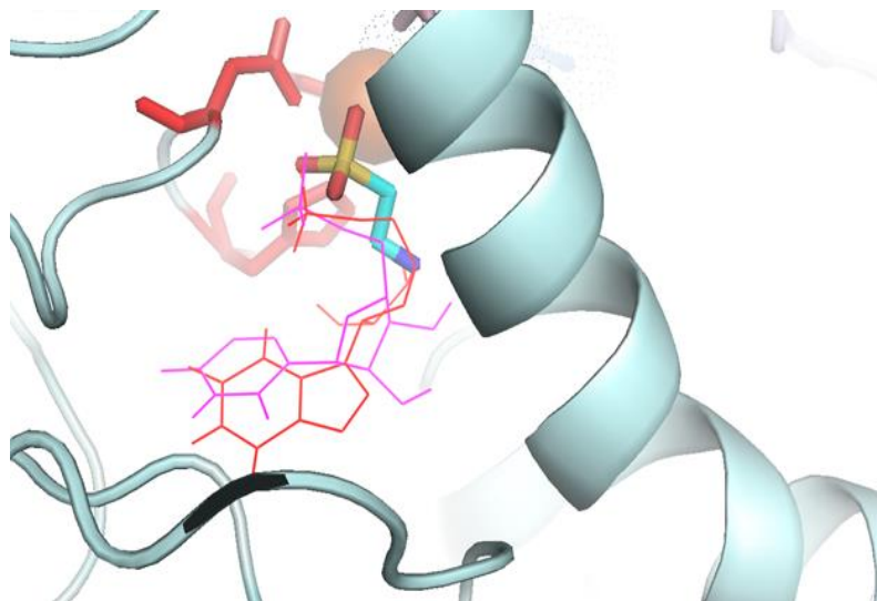
Figure 3.3.8.5. Docked XMP in the predicted active site. XMP (in red ) overlaps primary substrate UMP (shown in pink ), which in turn resides close to taurine (in rainbow colors) in the active site. Amino acid residues involved in the facial triad are depicted as sticks that interact with the Fe(II) center in the background.
