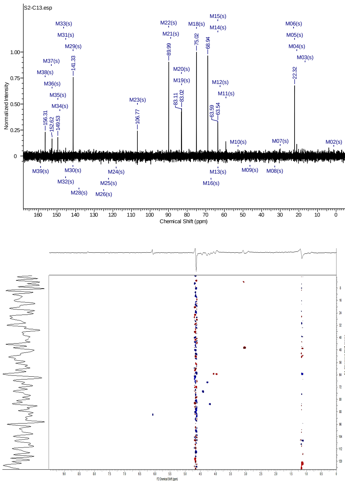
Figure 3.3.5.4. ^1\text{H} , ^{13}\text{C} , 2D ^1\text{H} - ^{13}\text{C} gHSQC (500MHz, \text{D}_2\text{O} ) for substrate analog S2.
