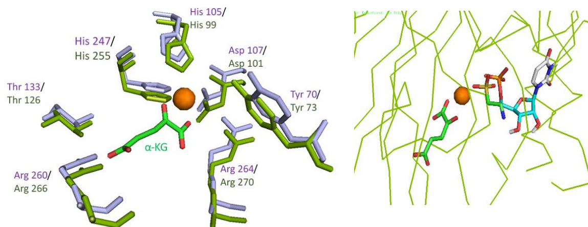
Figure 3.3.8.3. Overlay of the binding pocket of TauD (green) and Cpr19 (light blue). The active site amino acids that are conserved between the two enzymes are shown in green (TauD) and blue (Cpr19) (left). Docked UMP resides close to taurine in the TauD active site, and its phosphate moiety has a conformation similar to the sulfate group in taurine. Background ribbon shows surrounding protein structure (right).
