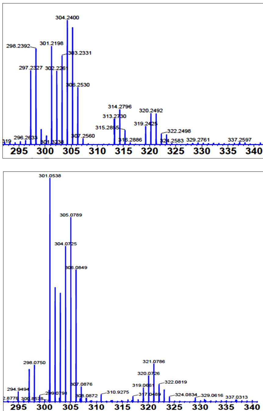
Figure 3.3.7.2. HRMS analyses for product peaks collected from reactions starting from XMP (A), S2 (B), S3 (C) and S4 (D). (A) HRMS (ESI+) calcd. for C_{10}H_{10}N_4O_6 [M + H]^+ 283.0634; found 283.0650; (B) HRMS (ESI+) calcd. for C_{10}H_{10}N_4O_6 [M + H]^+ 283.0634; found 283.0884; (C) HRMS (ESI+) calcd. for C_{10}H_{10}N_4O_7 [M + H]^+ 298.0549; found 298.2392; (D) HRMS (ESI+) calcd. for C_{10}H_{10}N_4O_7 [M + H]^+ 298.0549; found 298.0750.
