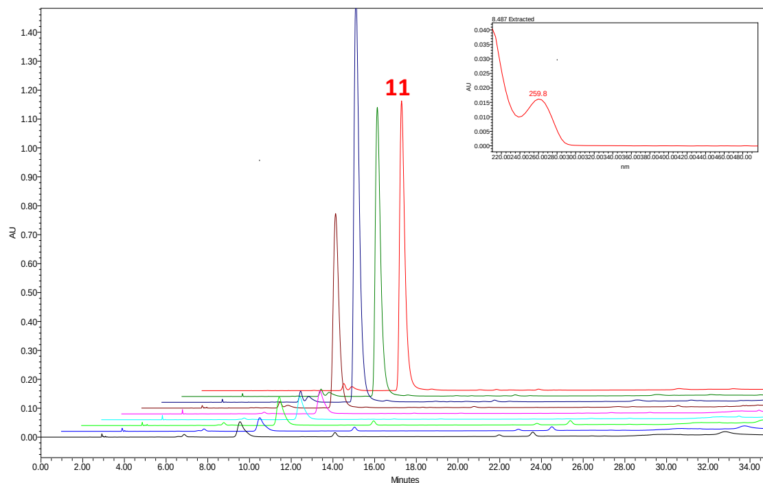
Figure 2.5.4.1. Reaction of LipL with S11. Comparative HPCL analyses of reactions carried out with phosphonate substrate analog 11 with LipL, under variable concentrations of 11 . The observed peak corresponds to unutilized 11 in reaction. None of these studies yielded a product peak. Inset: Absorbance maxima at 260 nm.
