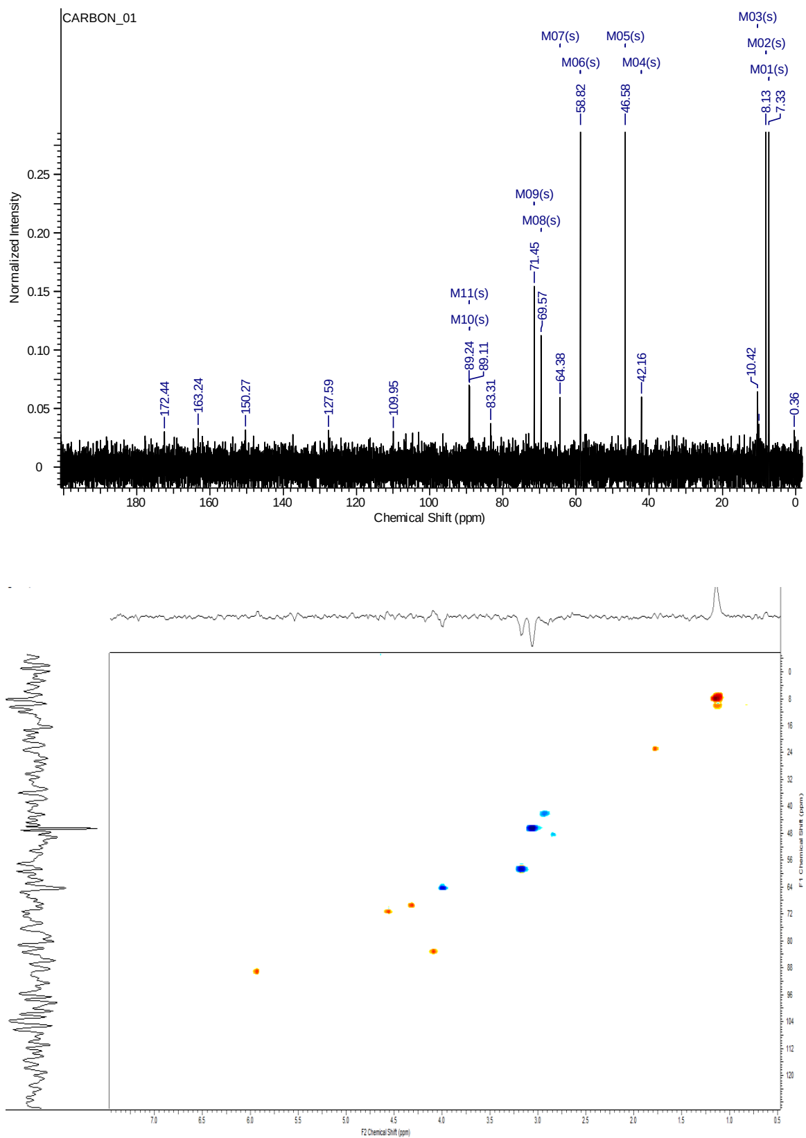
Figure 3.3.5.6. ^1\text{H} , ^{13}\text{C} , 2D ^1\text{H} - ^{13}\text{C} gHSQC (500MHz, \text{D}_2\text{O} ) for substrate analog S4.
