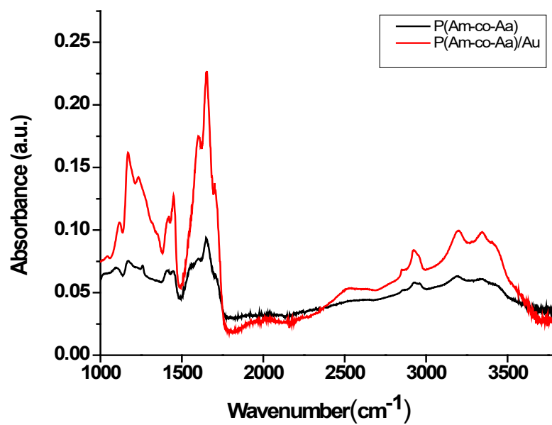
Figure 9 FTIR analysis for plain copolymer and copolymer with 250 \mu L Au-Np's.
