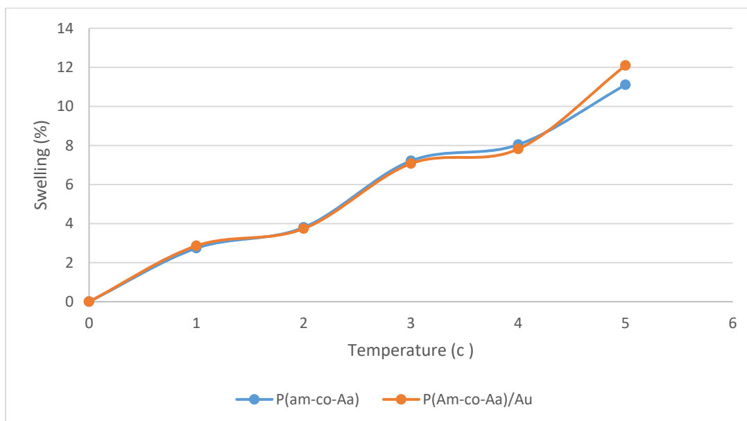
Figure 16 Modified and plain hydrogels average swelling temperature. T 1 = [20-30]°C, T 2 = [30-40]°C, T 3 = [40-50]°C, T 4 = [50-60]°C, T 5 = [60-70]°C.
