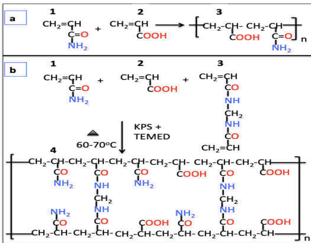
Figure 10 Possible hydrogel molecular structure. a1, b1) Acrylamide (Am). a2, b2) Acrylic acid (Aa), a3) P(Acrylamide-co-AcrylicAcid), P(Am-co-Aa). b3) N,N' Methylenebis (acrylamide)(MBAA).b4) cross-linked P(Am-co-Aa), Degree of polymerization (n), Potassium persulfate (KSP), N,N,N',N'-Tetramethylenediamine (TEMED).
