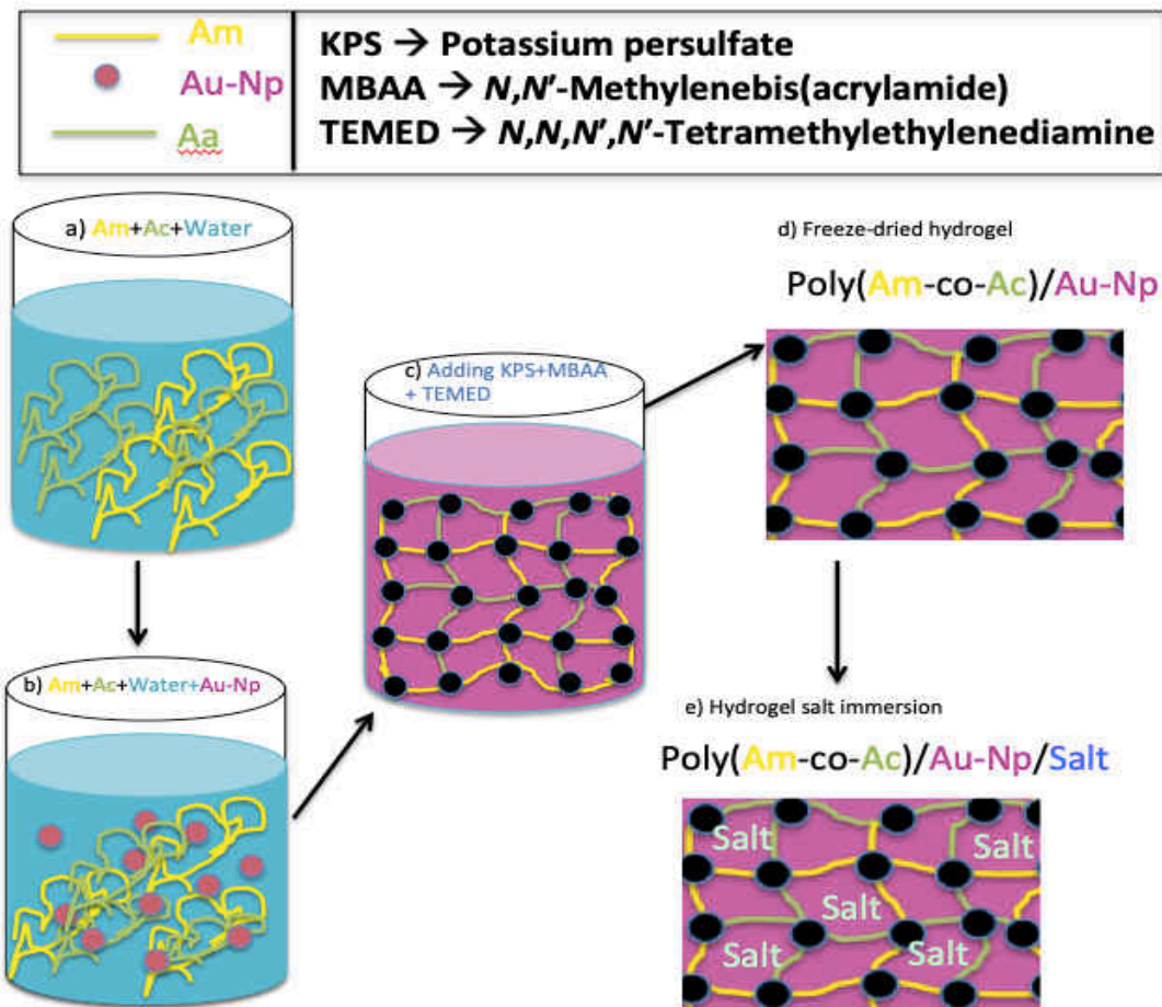
Figure 4 .Polymerization summary.
