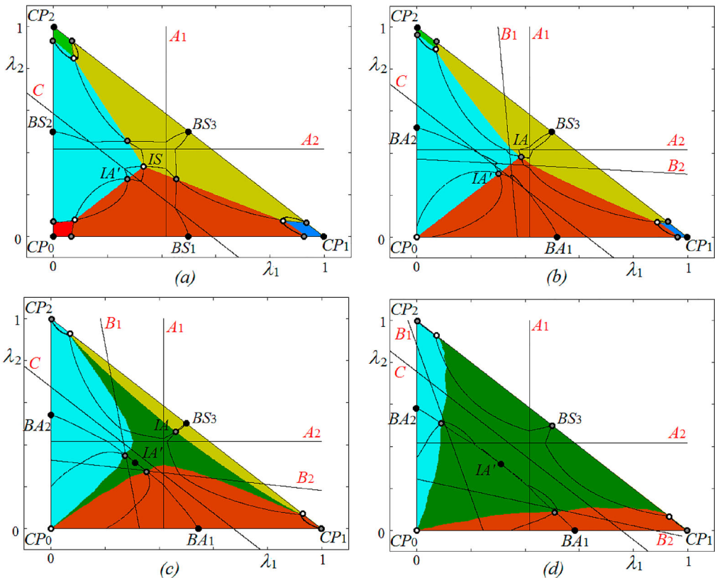
Figure 4. Basins of coexisting attracting fixed points of map Z for T_U = 0.325, L = 20 and T_{EX} = 0.325 in (a); T_{EX} = 0.35 in (b); T_{EX} = 0.38 in (c); and T_{EX} = 0.45 in (d). The related parameter points are marked in Figure 3(a) by black circles along the arrowed line drawn at L = 20 . The other parameters are fixed as in (17).
