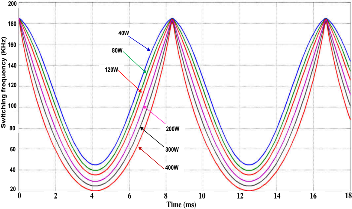
Figure 4.4 Switching frequency versus load range variation at a line period of output current
