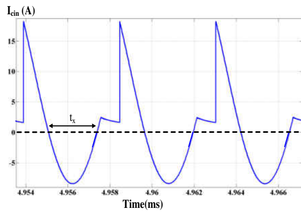
Figure 5.2 Input capacitor current with various switching frequency at 400W output and different input voltage: (a) f_s = f_r ; (b) f_s > f_r ; (c) f_s < f_r
