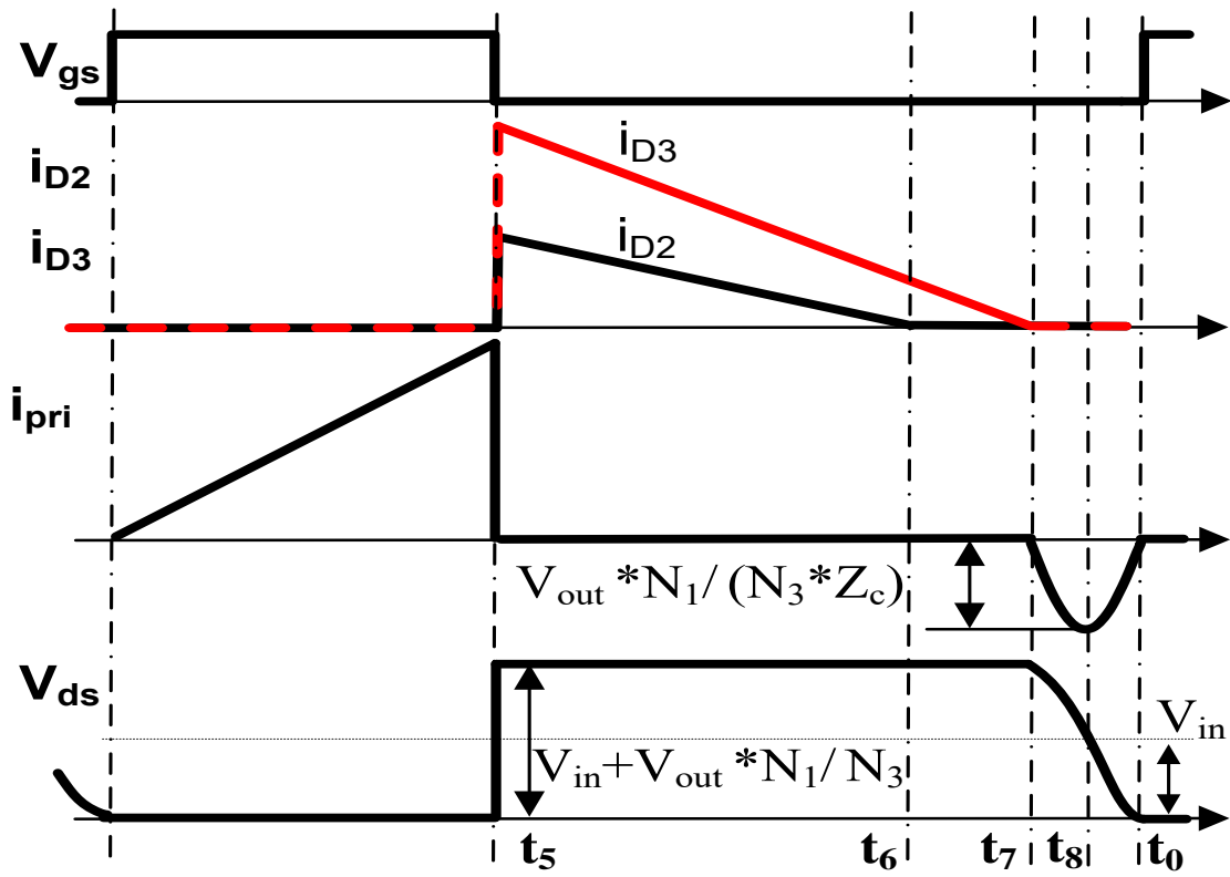
Figure 2.8 Key waveforms of BMFFC during off time
