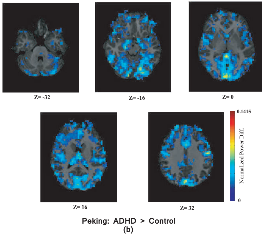
Figure 6.13: Plots of the average power differences of the control and ADHD groups on the subjects of Peking released and hold out set on different brain slices. (a) shows the regions where control group has higher power, (b) shows the regions where ADHD group has higher power.
