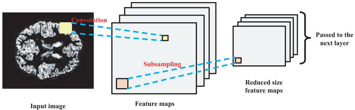
Figure 6.1: Figure shows the functionality of a CNN layer. First the input is convolved by a set of filters to produce the feature maps. Next the subsampling of the feature maps helps to reduce the map dimension. The reduced feature maps are then passed to the next layer for processing.
