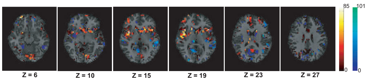
Figure 4.9: The figure shows the average differences of the degrees between the control and ADHD groups in the voxels belonging to the useful region mask. The average differences are calculated for the 83 subjects of the KKI released set. The dark red to white color map is used to represent the regions with higher degrees in control subjects and blue to green color map is used to show the opposite. The control group shows higher connectivity in the Cingulate Gyrus ( Z = 10, 15 ) and Paracingulate Gyrus regions ( Z = 19, 23 ).
