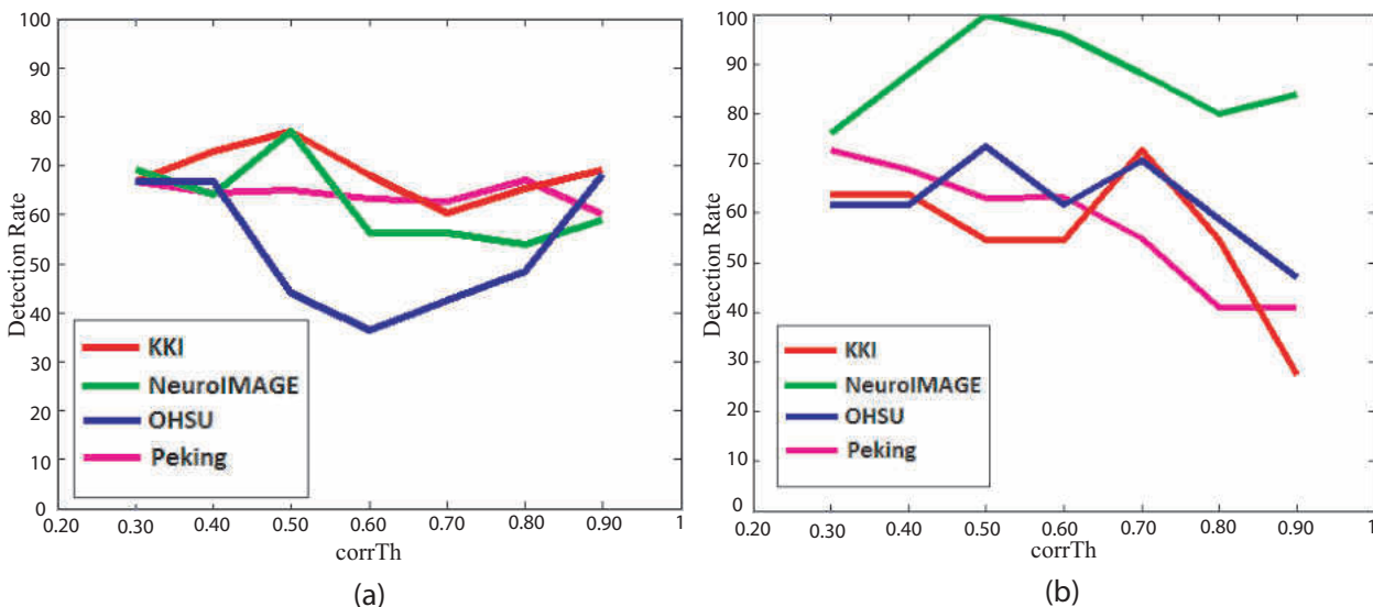
Figure 5.2: Figure plots corrTh vs detection rates of our method on the (a) released sets and (b) holdout sets.
