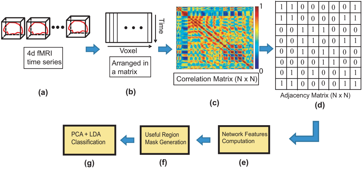
Figure 4.1: Overview of our approach: (a) given the 4-d fMRI data for a subject, (b) first we rearrange it as a matrix. (c) Next, a correlation matrix of size N \times N ( N is the number of voxels) is computed. (d) An adjacency matrix is generated after thresholding the correlation values into binary numbers. The adjacency matrix represents a network. (e) Network features such as the node degree and cycle count for each node of the network are computed. (f) Next, we generate the useful region mask. (g) Feature values from the nodes, identified by the useful region mask, are used to form the feature vector and a PCA-LDA classifier is used for the classification.
