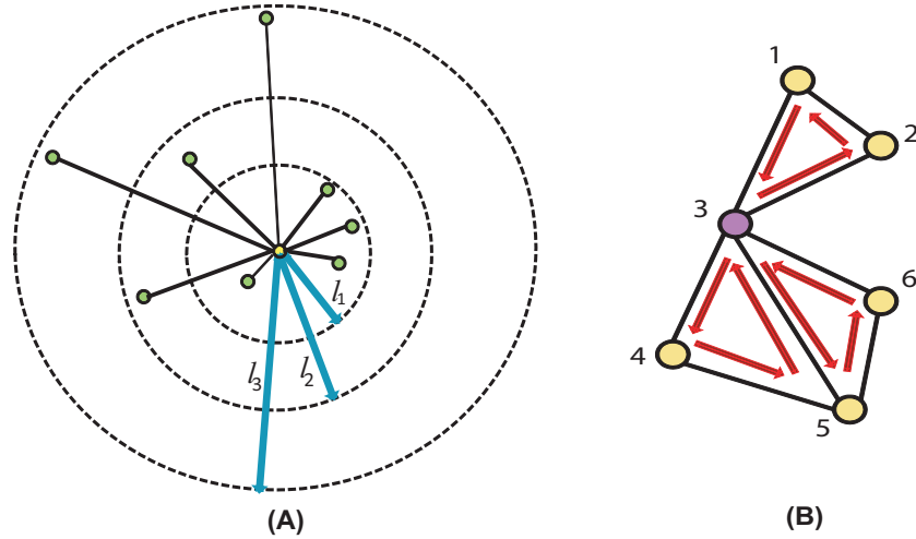
Figure 4.2: (A) The degree of the node, highlighted in yellow, is the count of all the green nodes connected to it (i.e. 8), while the varying distance degree is the counts of all the connected nodes in each of the bins defined by the three edge length thresholds ( l_1, l_2, l_3 ) showed by the blue arrows. In this example the varying distance degrees of the yellow node are \{4, 2, 2\} . (B) Shows all the distinct 3-cycles that contain node 3.
