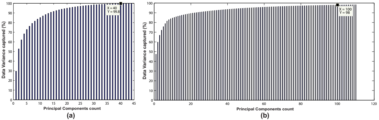
Figure 4.7: The figure shows the plots of principal component count vs percentage of data variance for (a) KKI released set (b) full released data of 776 subjects.
