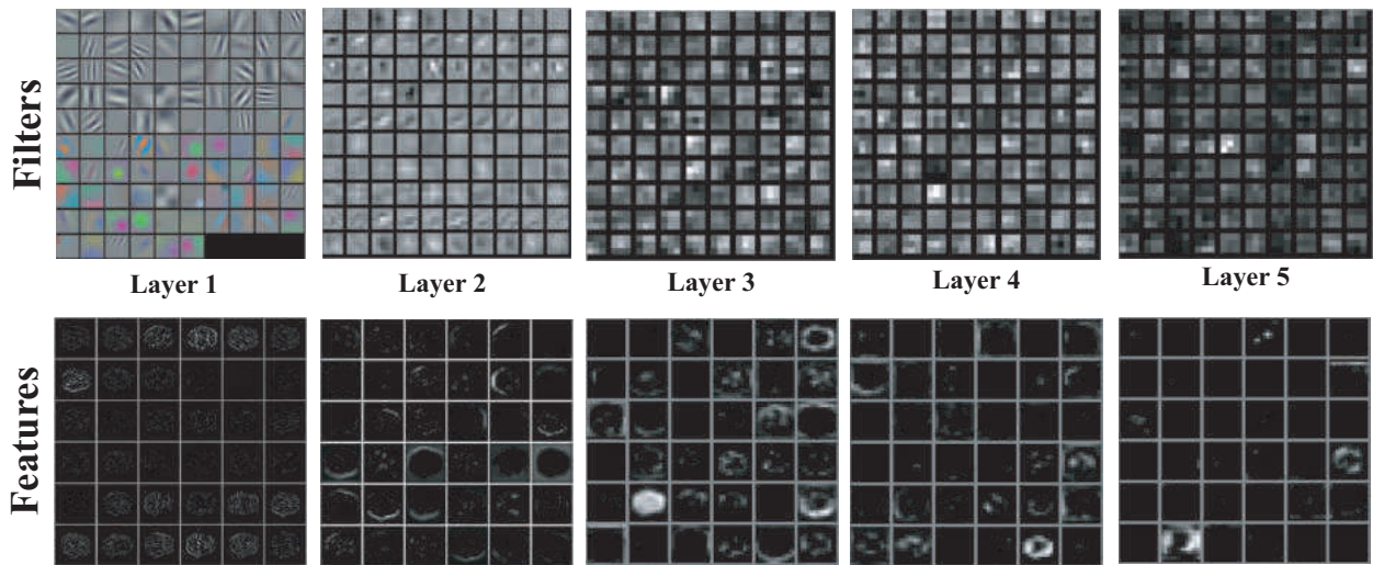
Figure 6.4: Figure shows some of the filters learned by the pre-trained CNN model for all five convolution layers and the corresponding feature maps generated for some input subject. Note that due to the space constraint, the figure is showing only a subset of the filters and features of each layer.
