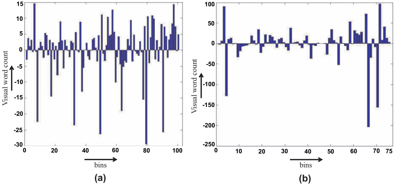
Figure 3.3: The figure shows the differences of average histograms of the control and ADHD group of subjects for (a) 4-tuple degree features and (b) raw intensity time series features.
