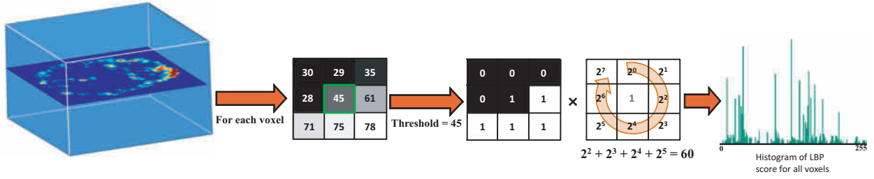
Figure 6.6: Figure describes the LBP feature computation on a 2-D image. First, for each voxel immediate 8 neighbour voxels in the plane direction are identified. Then, a neighbour voxel is assigned a value 0 if its power value is less the center voxel's value. Otherwise it is assigned a value 1. Next, the binary values of all the neighbour voxels are multiplied by different powers of 2 in a particular order and summed. This is the LBP score of the center voxel. Finally, the histogram of LBP scores is computed for all the voxels of the brain volume under consideration.
