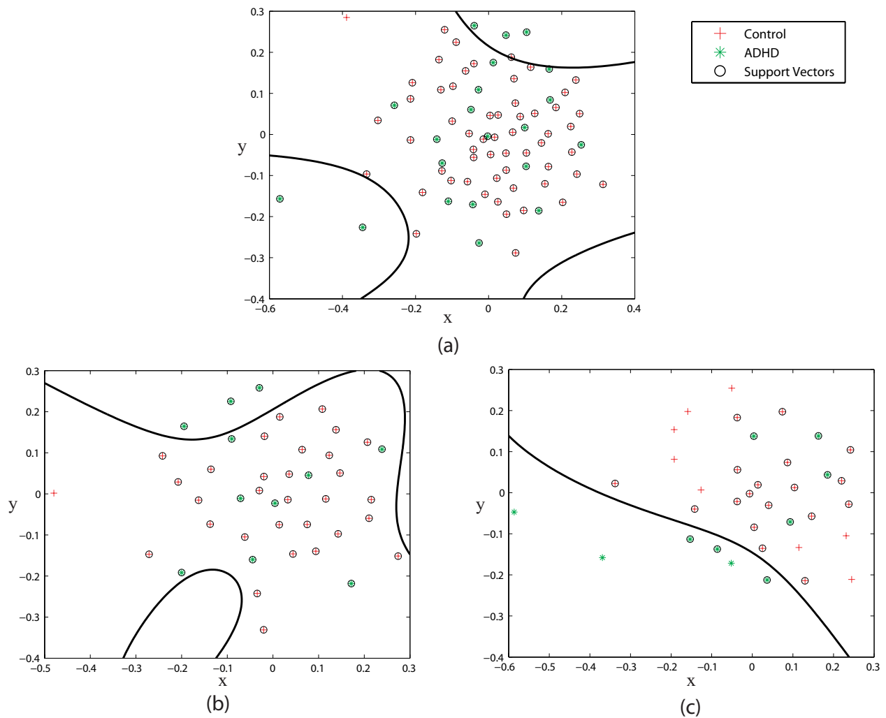
Figure 5.5: Subjects from the KKI released set are plotted on the MDS projected space. (a) All subjects, (b) subjects of the male group, (c) subjects of the female group. The spaces are segmented during the SVM training phase.
