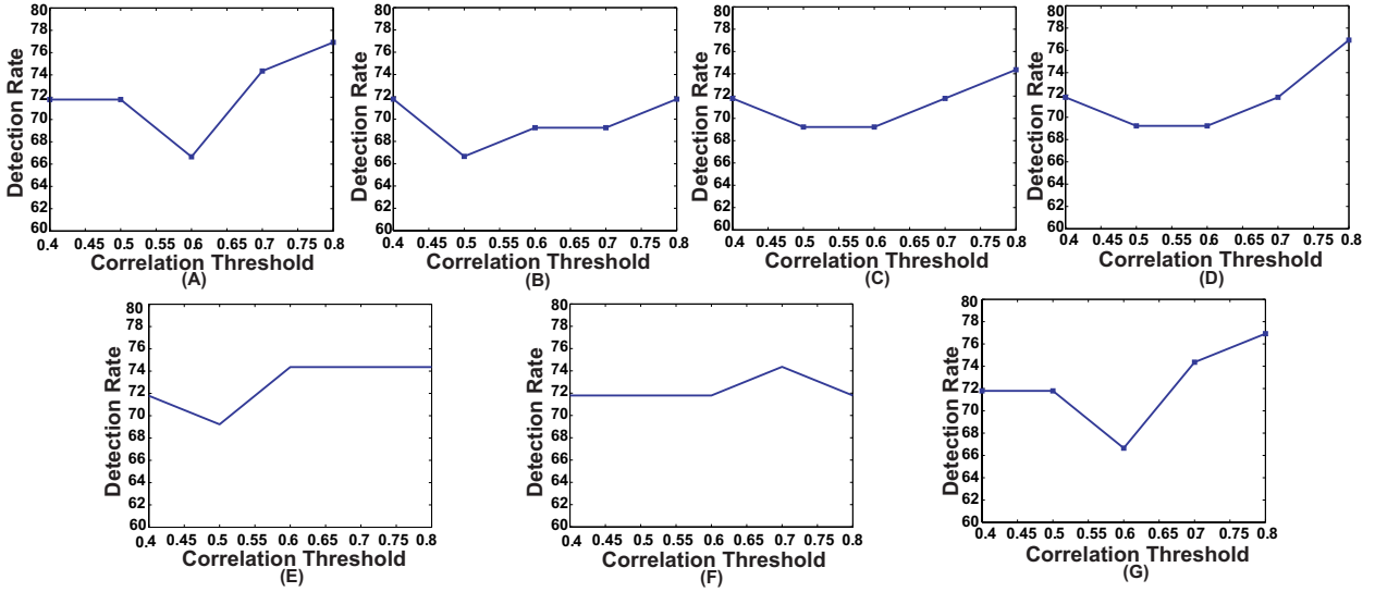
Figure 4.6: The plots show how detection rates for different network features change with correlation threshold. (A) Degree map positive correlations, (B) degree map negative correlations, (C) degree map absolute correlations, (D) varying distance degree map positive correlation, (E) 3 cycle map positive correlation, (F) 4 cycle map positive correlation, (G) weight map positive correlation.
