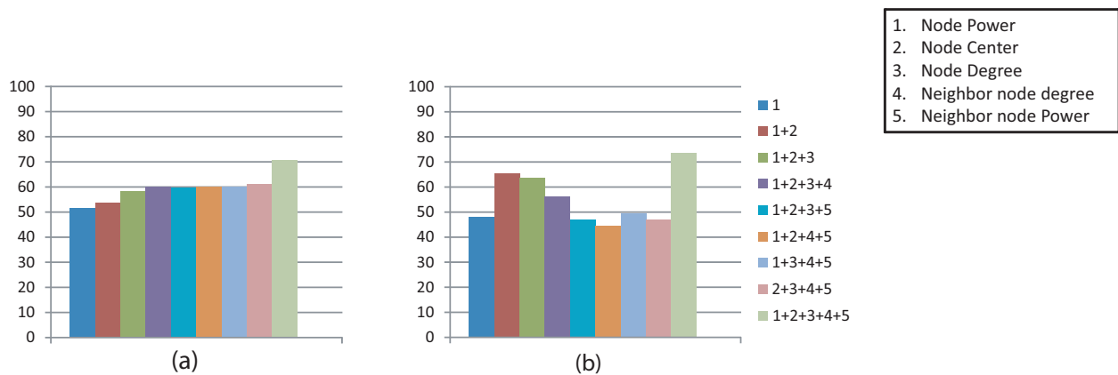
Figure 5.4: Figure plots the average detection accuracies on all the data centers when the inter-graph distances are computed using different subsets of the node attributes. The classification is performed on the male and female groups of subjects separately to achieve the reported results on (a) the released sets and (b) holdout sets.
