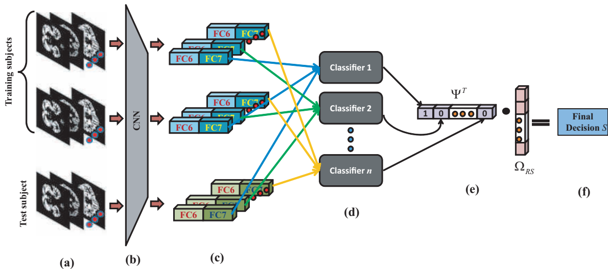
Figure 6.3: Flowchart of the GM classification framework: (a) GM images of the training and test subjects are provided to a pre-trained CNN (b) to extract features from FC6 and FC7 layers. (c) For separate slices, separate feature vectors are constructed concatenating the features from the FC6 and FC7 layers. (d) Separate classifier are trained for the separate slices to produce the decision vector \Psi . Dot product of \Psi and a weight vector \Omega_{RS} generates the final decision score S .
