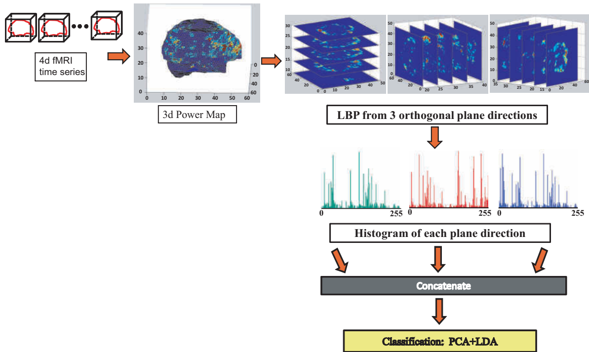
Figure 6.5: Flowchart of the power map classification framework: First, the 3-D power map image is generated from the 4-D fMRI data. Next, the LBP texture features are computed in three orthogonal plane directions of the power map image. The classification is performed using the PCA-LDA classifier.
