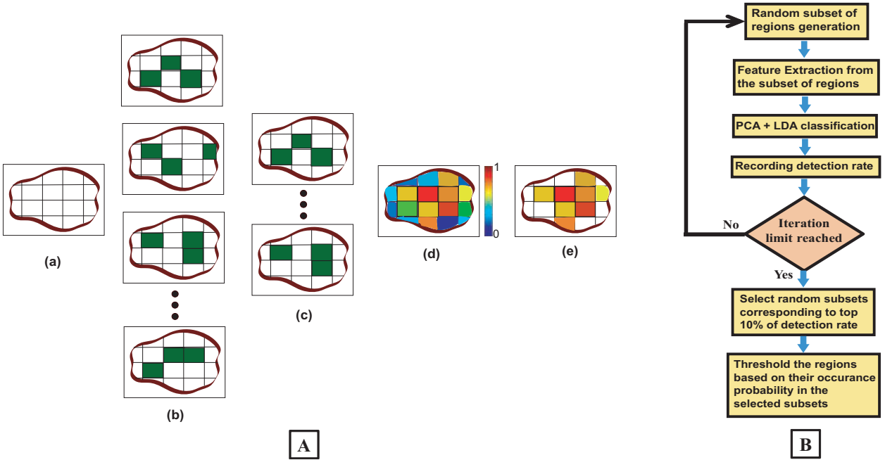
Figure 4.3: (A) This part of the figure explains the useful region mask generation algorithm on a single brain slice. The figure is just a graphical example, not the real data. In the actual experiments the brain volumes are used instead of slices and volumetric regions are used instead of square subdivision areas. (a) Divide the slice into square regions. (b) Select random sub sets of the regions marked in dark green. (c) Select the sub sets with top 10% of detection rate. (d) Generate a probability map based on the regions occurrence in top 10% subset. (e) Threshold the probability map to produce the useful region mask. (B) This part shows the flowchart for the mask generation algorithm.
