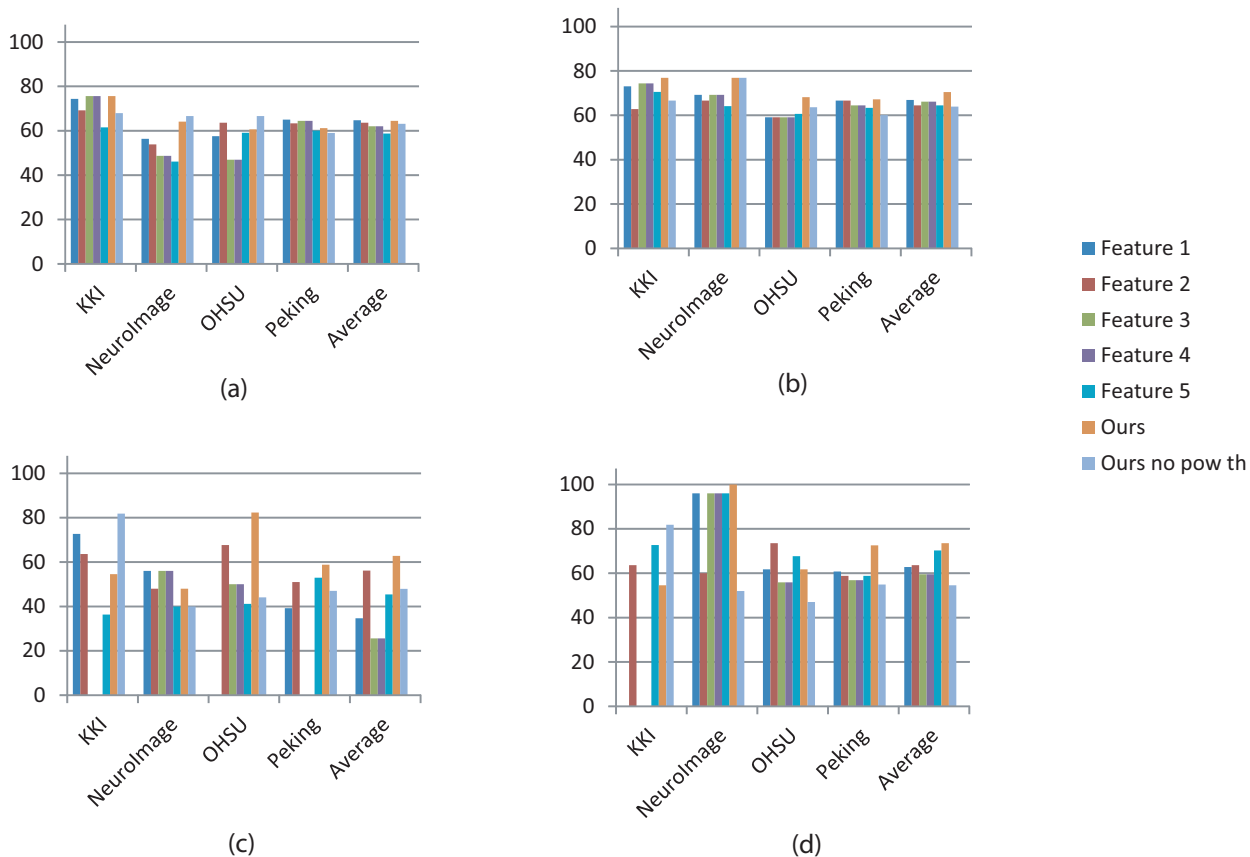
Figure 5.3: Summary of the results: figure plots the best detection rates achieved on all the released and holdout sets using five commonly used network features implemented in the BCT, our method and our method without the high power voxel selection step. Features 1 to 5 are the degree, topological overlap, clustering coefficient, local efficiency and rich club coefficient respectively. (a) and (b) show the results on the released sets when the classification is performed on all the subjects and on the male and female subjects separately. (c) and (d) show the similar results on the holdout sets. The detection rates of (b) and (d) are computed by averaging the detection rates on the male and female groups.
