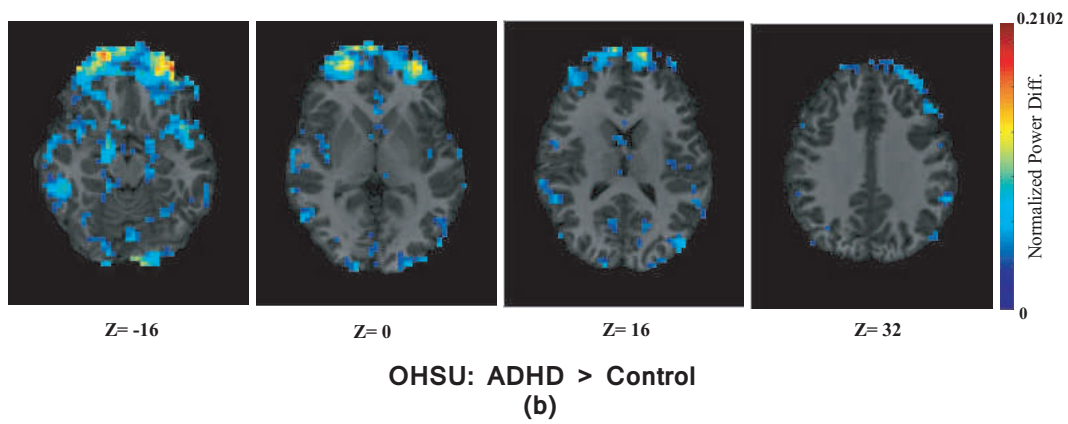
Figure 6.12: Plots of the average power differences of the control and ADHD groups on the subjects of OHSU released and hold out set on different brain slices. (a) shows the regions where control group has higher power, (b) shows the regions where ADHD group has higher power.
