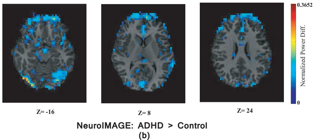
Figure 6.10: Plots of the average power differences of the control and ADHD groups on the subjects of NeuroIMAGE released and hold out set on different brain slices. (a) shows the regions where control group has higher power, (b) shows the regions where ADHD group has higher power.
