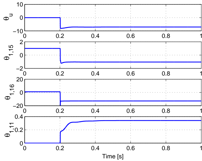
Figure 2.17: Time evolution of sample parameter estimates at pre-flutter speed V_\infty = 2.26 < V_f
