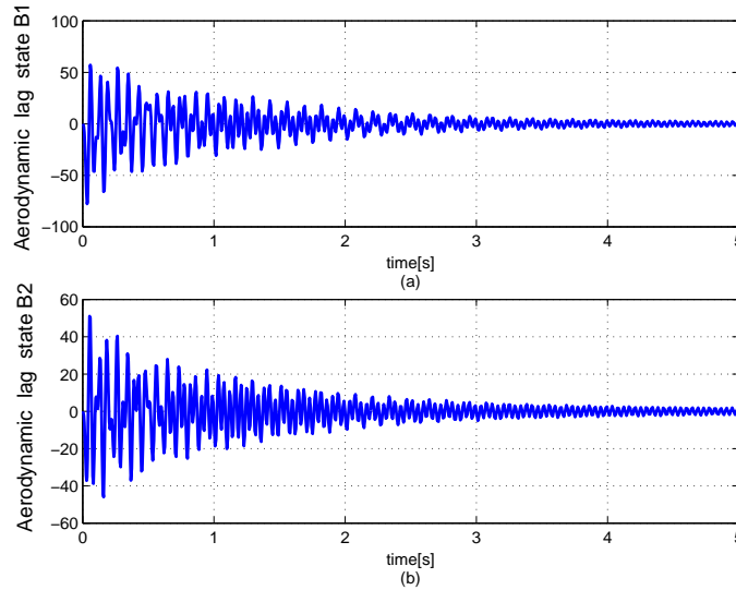
Figure 2.3: Open-loop aerodynamic lag states B_1, B_2 pre-flutter speed V = 0.8V_f
