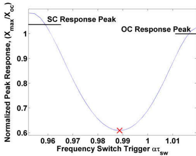
(b) The peaks of each response (red dots in Fig. 4.4a) mapped to their frequency-based switch triggers, with optimal trigger (red X)
