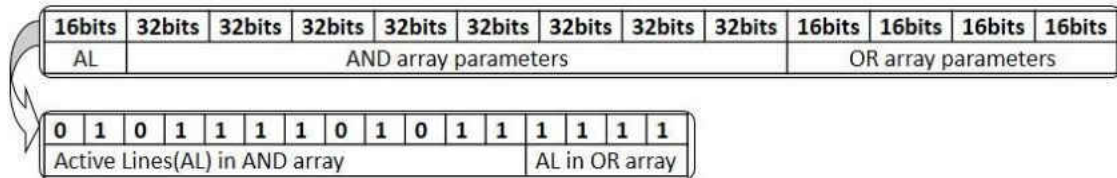
Figure 11: Chromosome representation for each UDB evolved in DDC
