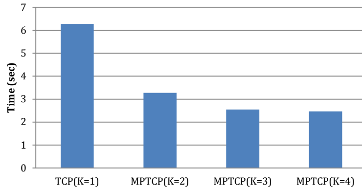
Figure 7-3: Arrival rate = 2 bursts/ \mu s, W=64
