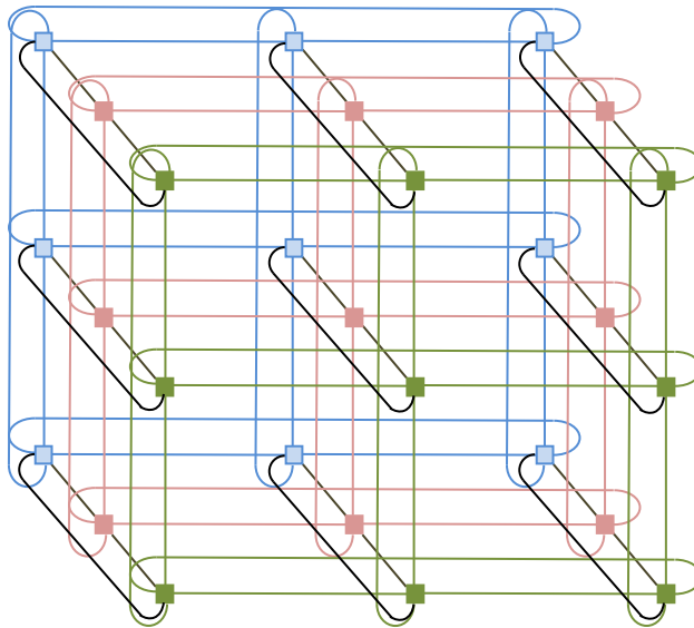
Figure 9-4 3x3 6D Mesh Torus
