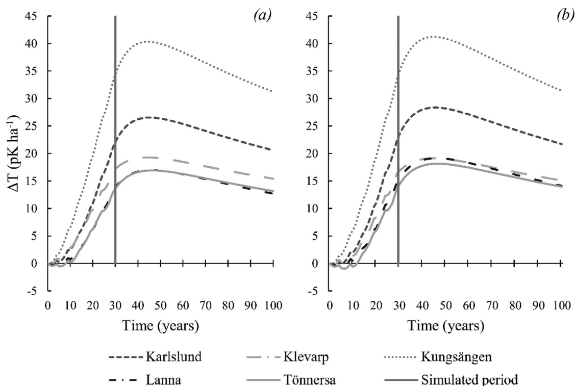
Figure 6. Simulated potential temperature response of the grass cultivation system during the 30-year study period with fertilisation rate (a) F1 (140 kg N \text{ha}^{-1} ) and (b) F2 (200 kg N \text{ha}^{-1} ) at the five study sites. The temperature response is expressed as \text{pK ha}^{-1} ( p = 10^{-12} , K = Kelvin).
