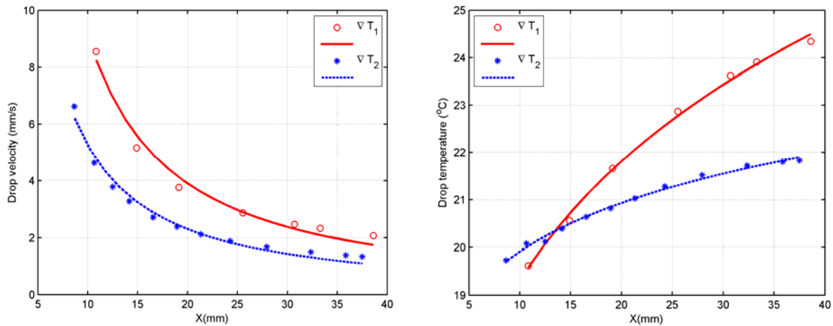
Figure 38 Lens droplet (4 \mu L) velocity (left) and temperature increase (right) for two thermal slopes.
