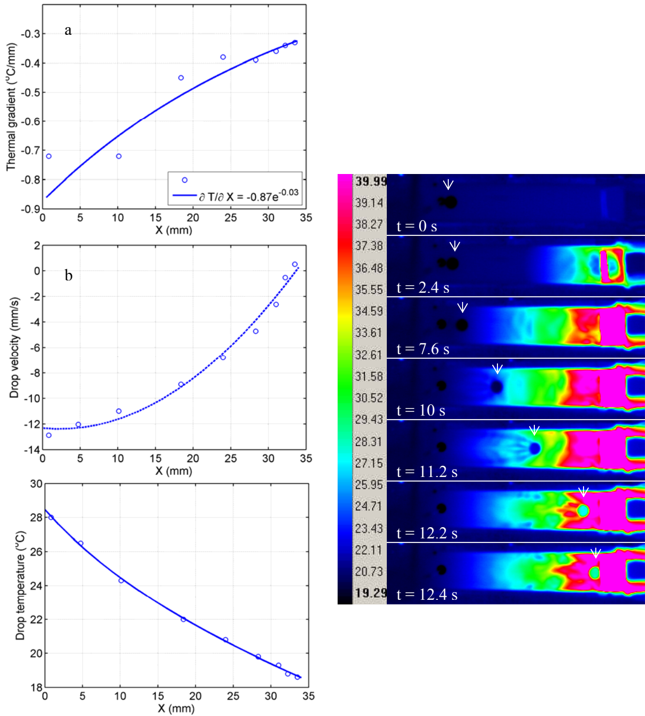
Figure 39 Motion of a spherical drop ( 14 \mu\text{L} ) due to a transient thermal field. Left a) thermal gradient felt by the drop along the path b) instantaneous drop velocity c) change of drop temperature. Right column shows the infrared images at select times.
