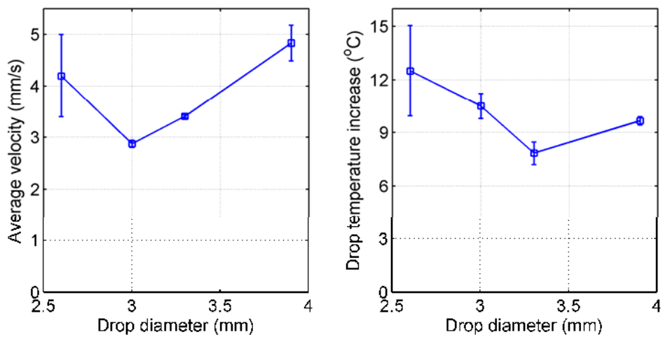
Figure 42 Effect of drop size on average drift speed and overall increase in drop temperature as it moves across the platform.
