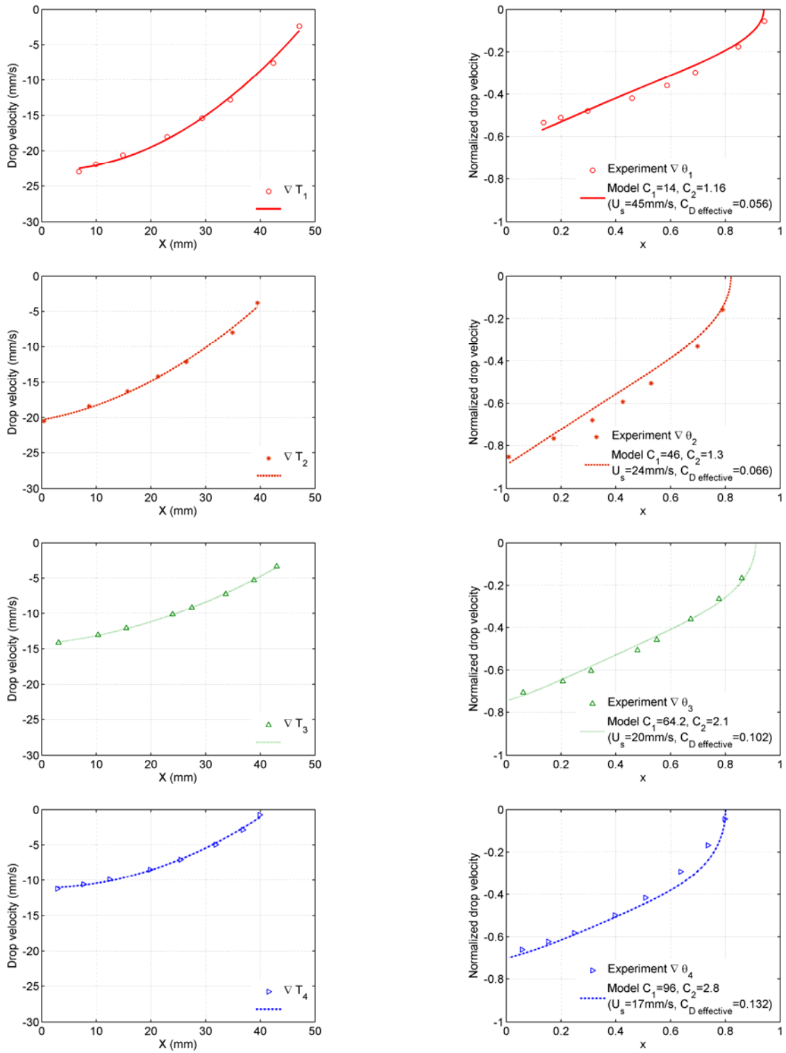
Figure 47 Drop (spherical) velocity from experiment is compared by drop velocity calculated from the proposed model (effective drag C_{D\text{ effective}} varies from 0.0566 to 0.132 for various cases)
