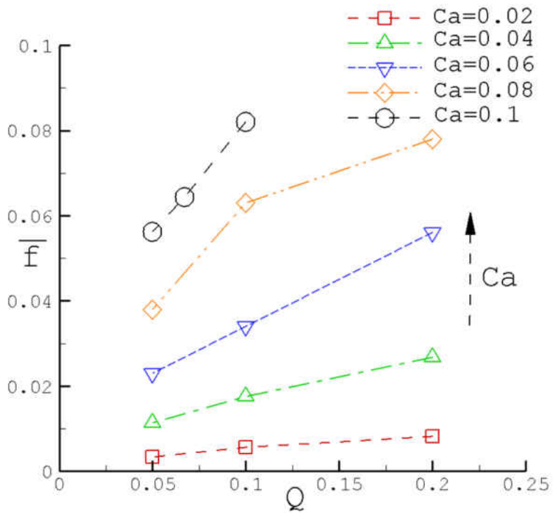
Figure 47: Dimensionless frequency of droplet formation for various Capillary numbers in the transition regime.
