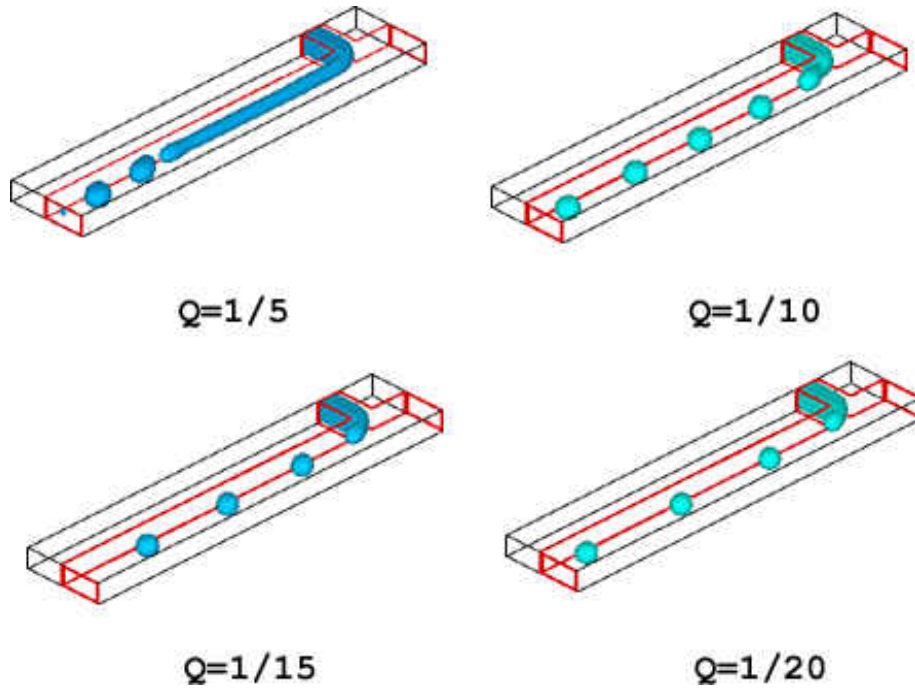
Figure 48: Flow regimes for \Lambda = 1/2 and Ca=0.1 at different flow rate ratios.
