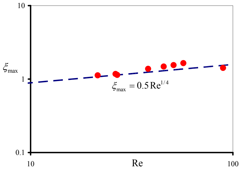
Figure 30: (a) Comparison of LBM simulation results (●) with (a) experiments and correlation of Scheller (---, \Delta ), Asai ( \square ) and correlation of Pasandideh-Fard ( \diamond ). (b) Comparison of LBM (●) with the analytical solution of Pasandideh-Fard (---).
