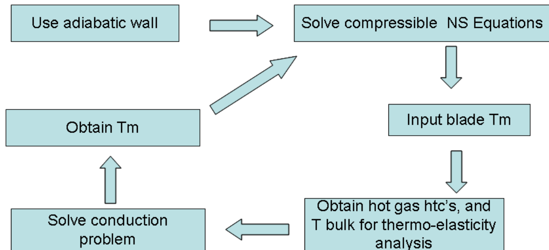
Figure 5: External loop
