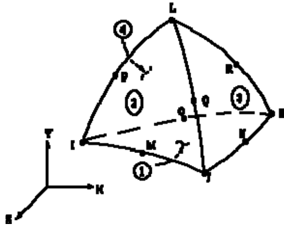
Figure 13: Solid92 geometry
