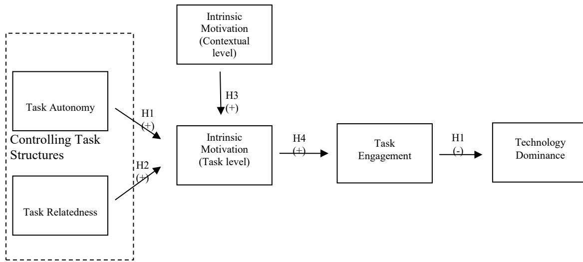
Figure 4-1: Theoretical Model
