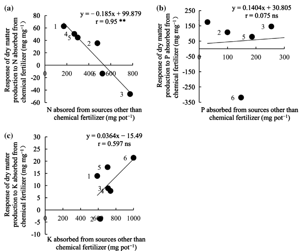
Figure 4. Relationships between N, P, and K absorbed from sources other than chemical fertilizer and responses of dry matter production to N, P, and K absorbed from chemical fertilizer. Numbers on the left of dots represent the numbers of the soils for pot experiment. Note. **significant at P < .01 ; ns, not significant.
