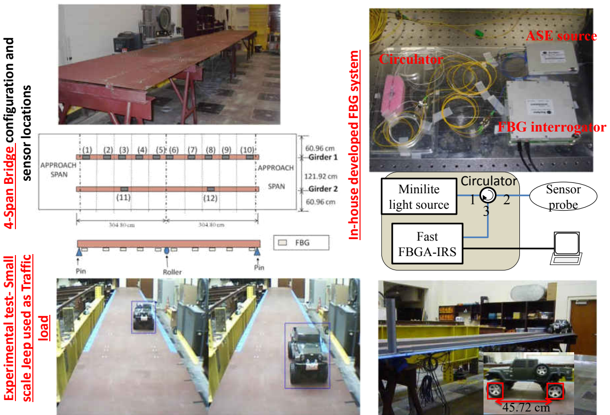
Figure 13: UCF-4 Span Bridge used for experimental test
