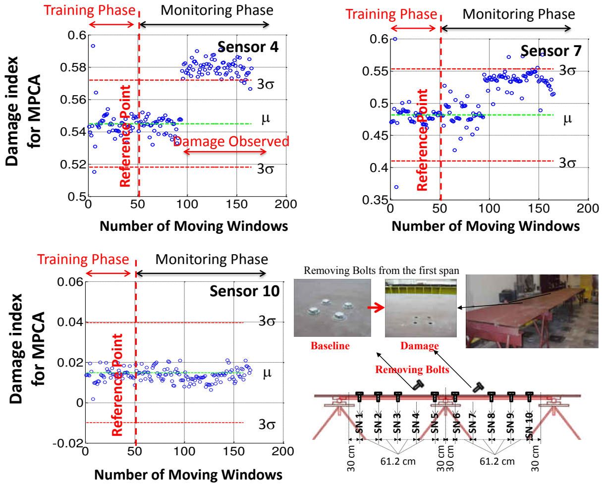
Figure 33: MPCA results for selected sensors (case5)
