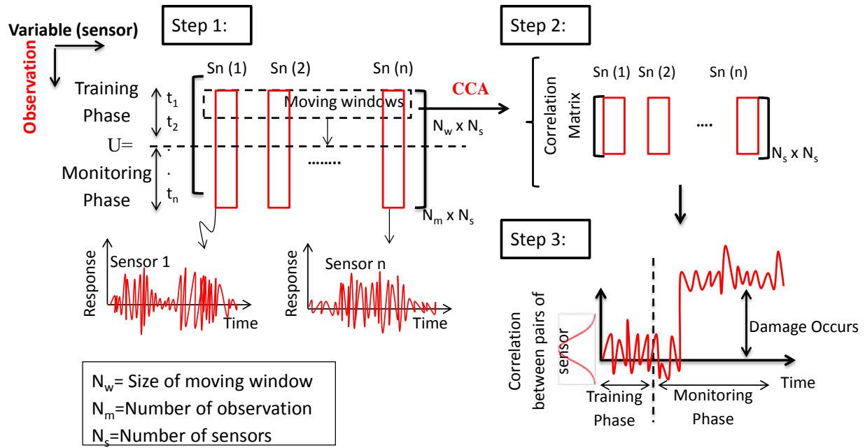
Figure 9: Procedure for Moving Cross Correlation Analysis (MCCA)
