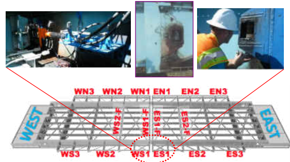
Locations of the Induced Damages
