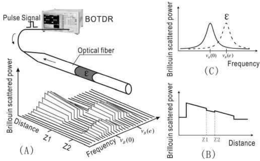
Figure 6: BODTR measurement principle [74]
