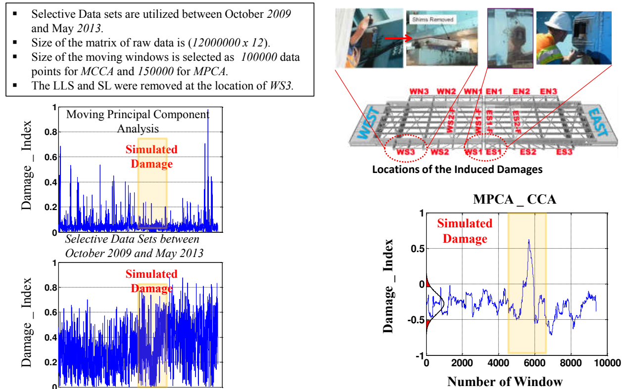
Figure 44: The corresponding results for case 2 (removing some of the shim from the span lock and live load shoe close to the location of WES3 and WS1 sensors)
