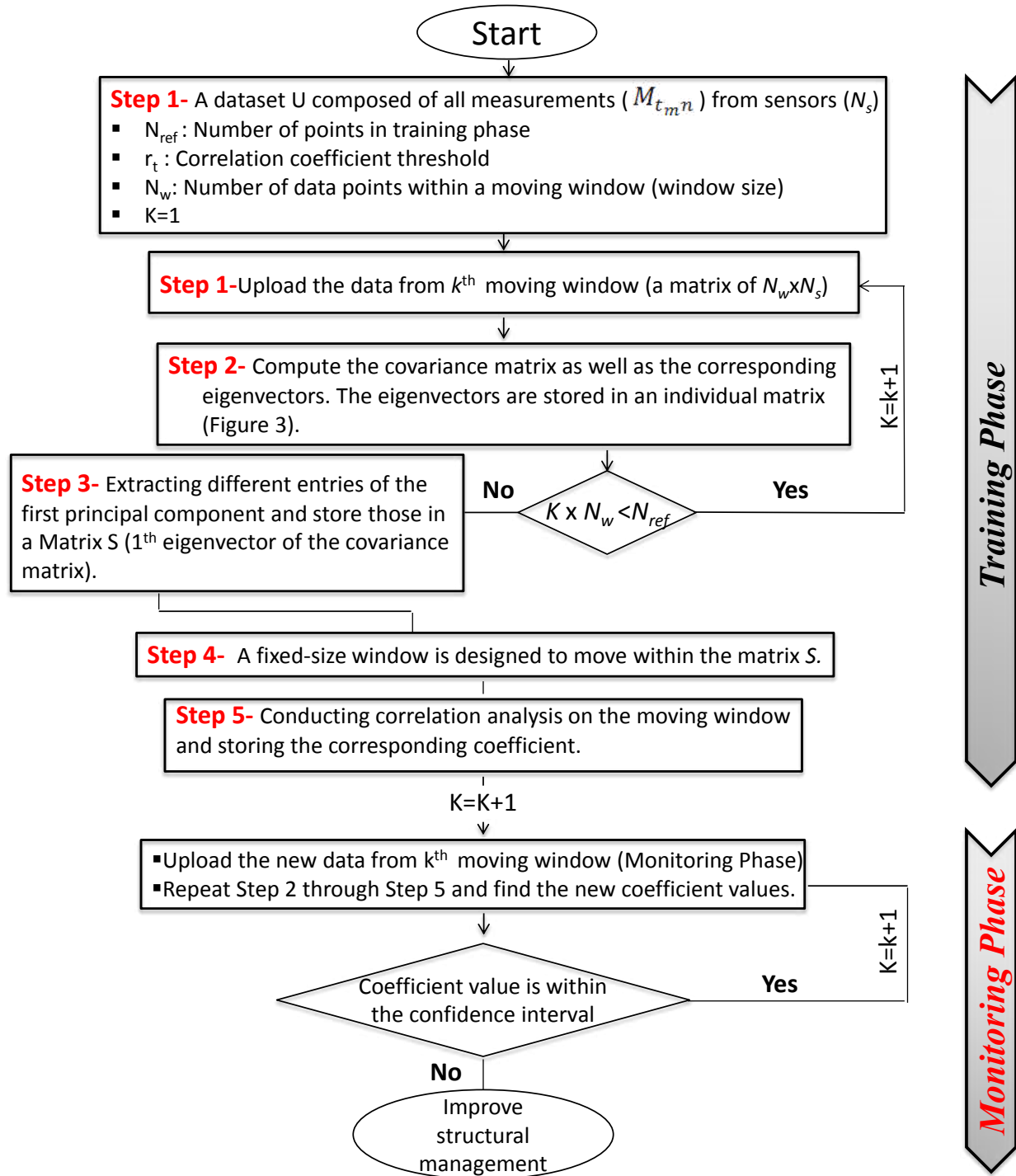
Figure 36: The sequential steps for conducting MPCA-CCA algorithm
