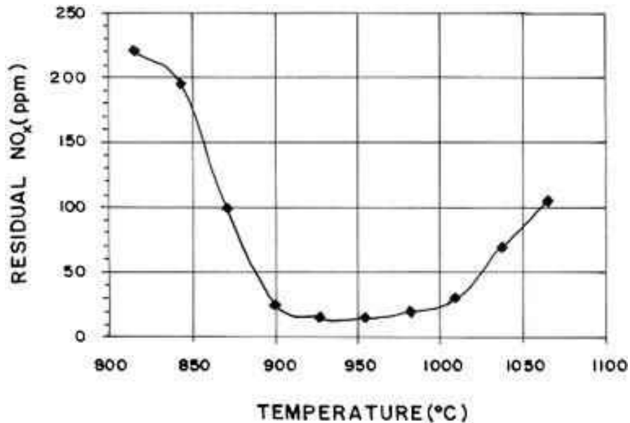
Figure 5 - Temperature window of SNCR process using ammonia at molar ratio (NH 3 /NO x ) = 1.5 (Lyon & Longwell, Selective non-catalytic reduction of NO x by NH 3 , 1976)
