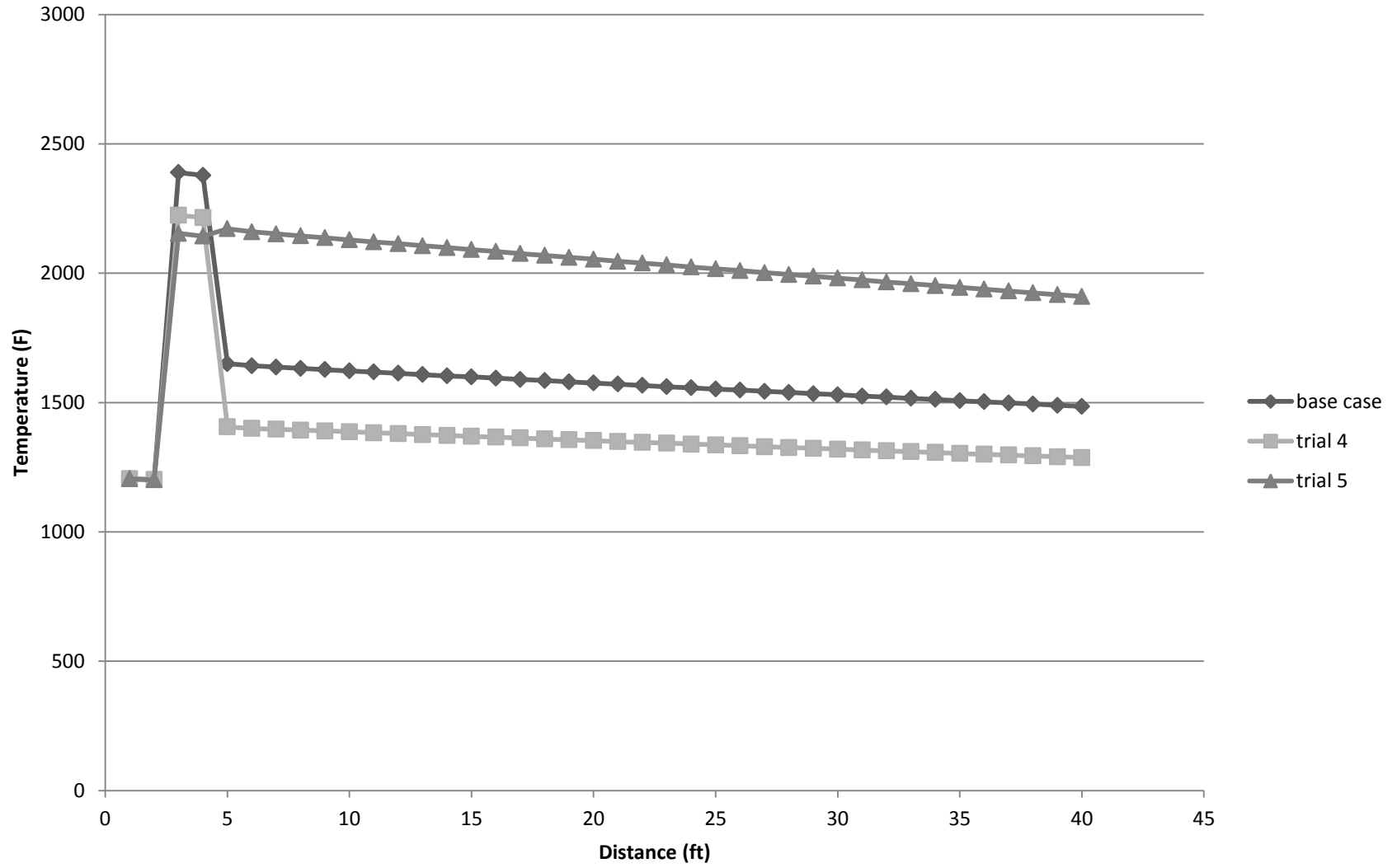
Figure 37 - temperature profile varying total air mass flow rate
