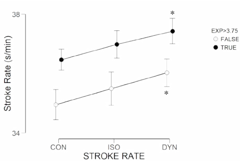
Figure 12: Mean stroke rate by testing condition and experience levels. Black circles represent high experience, and white circles represent low experience. * DYN>CON.
