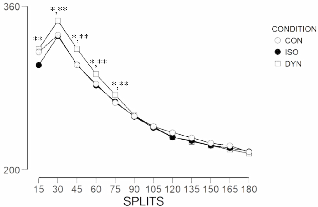
Figure 10: mean power analyzed by 15-second splits and categorized by condition. * DYN>CON.; ** DYN>ISO.
