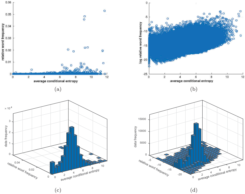
Figure 2. Top: the conditional entropy of contextual environments of words (horizontal axis) versus (a) relative word frequency, (b) logarithm of relative word frequencies. Bottom: the two-dimensional histograms of the conditional entropy of contextual environments of words and (c) the relative frequency of words, (d) the logarithm of relative word frequencies.
