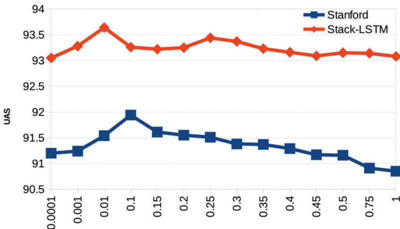
Figure 4. Vertical axis: unlabelled attachment scores obtained from parsing models trained with randomly initialised word vectors and gold part-of-speech tags. Horizontal axis: variance of the randomly generated vectors.
