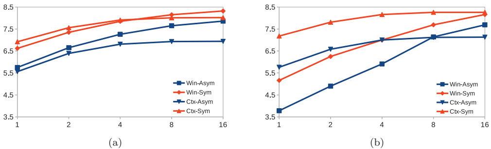
Figure 1. Vertical axis: the average conditional entropy of seeing a word given a context unit (a) before and (b) after context selection. Horizontal axis: the threshold value of n . Win: Window-based, Ctx: Context-based, Asym: Asymmetric, Sym: Symmetric.
