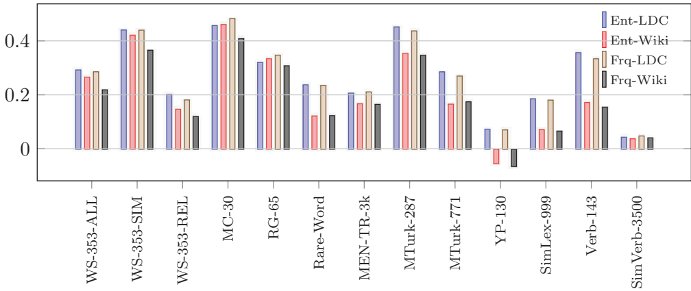
Figure 9. The breakdown results obtained from the word-similarity benchmarks with word vectors trained with the entropy-based feature selection (Ent) and the frequency-based feature selection (Frq). The word vectors are extracted from LDC and Wikipedia corpora. The x-axis shows the word-similarity benchmarks and the y-axis shows the correlation between word similarities. Each legend item shows a combination of context selection method (Ent or Frq) and the training corpus (LDC or Wiki).
