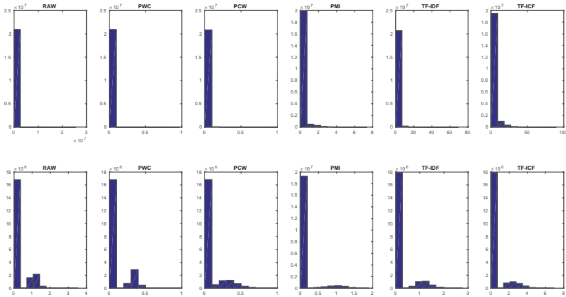
Figure 7. Data distribution (TOP) before and (BOTTOM) after performing power transformation.
