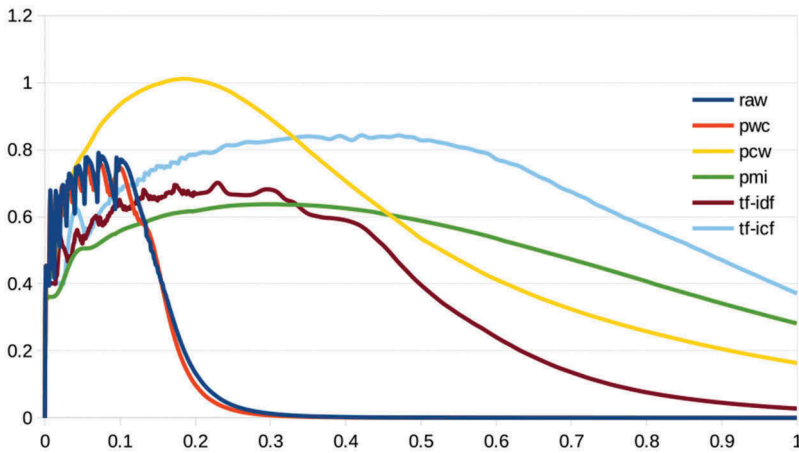
Figure 5. Behaviour of the functional in Equation (4) (vertical axis) with f = \sqrt[4]{x} and D = 1000 with respect to different values of \theta \in (0, 1] (horizontal axis).
