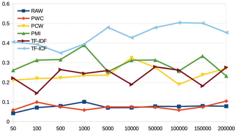
Figure 6. Optimal values of \theta (vertical axis) maximising the functional in Equation (4) for English with respect to different values of D (horizontal axis) and different global weighting functions.
