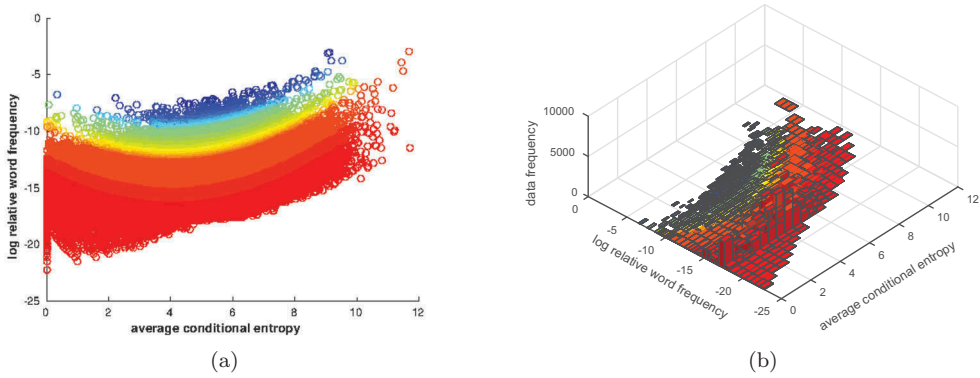
Figure 3. (a) The selected words after context selection with different values of D corresponding to the colour spectrum starting with D = 20 , dark blue, to D = 200\,000 , dark red. Horizontal axis: conditional entropy of contextual environments of words; Vertical axis: the logarithm of word frequencies. (b) The histogram of the selected words after context selection.
