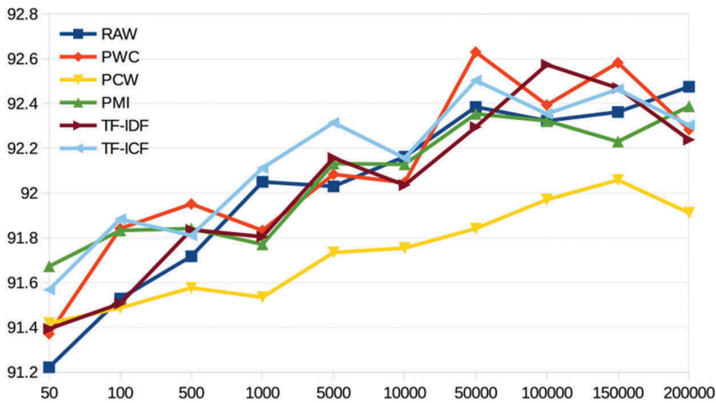
Figure 8. The effect of the number of context units (horizontal axis) and global weighting function on the parsing accuracy (vertical axis: UAS). The parsing models are trained evaluated on the development set of WSJ using gold part-of-speech tags.
