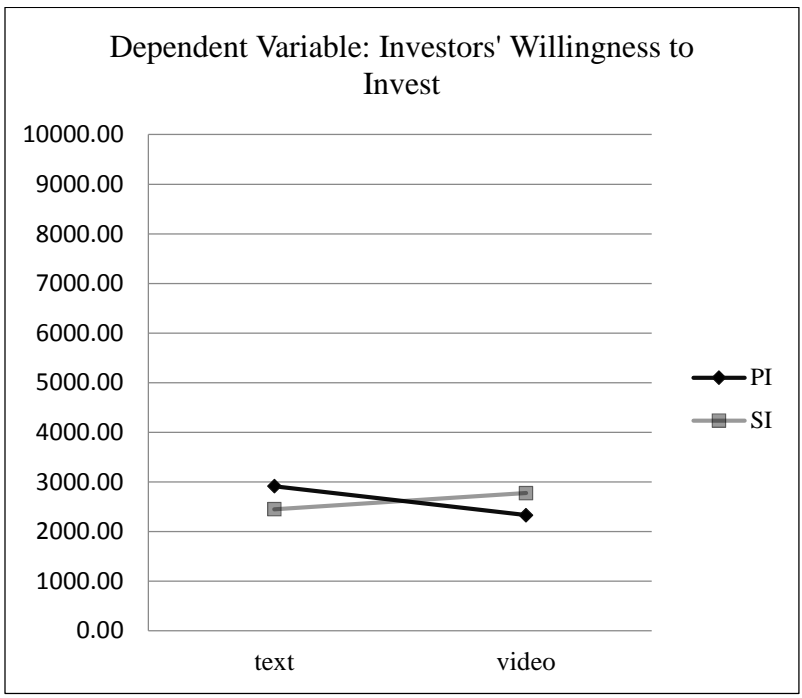
Figure 6: Expected Interaction
