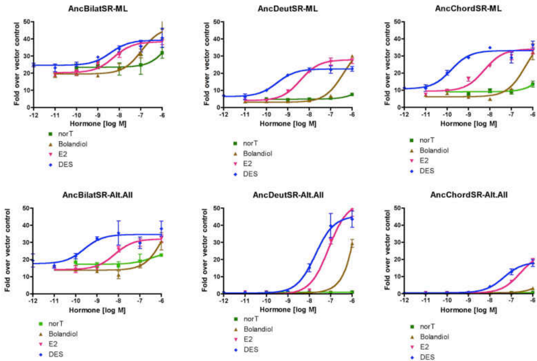
Figure S2. Dose response curves for ML and Alt.All ancestral SR LBDs reconstructed under the revised SR phylogeny including 14 newly discovered SRs and ERRs. Alt.All versions of SR LBDs include all alternate states for sites where the first alternate state has a posterior probability (PP) \geq 0.2 . Functions of ML and -Alt.All versions are qualitatively similar, except for alternate versions of AncDeutSR and AncChordSR, where the low level of constitutive activity observed in the ML versions is abolished.
