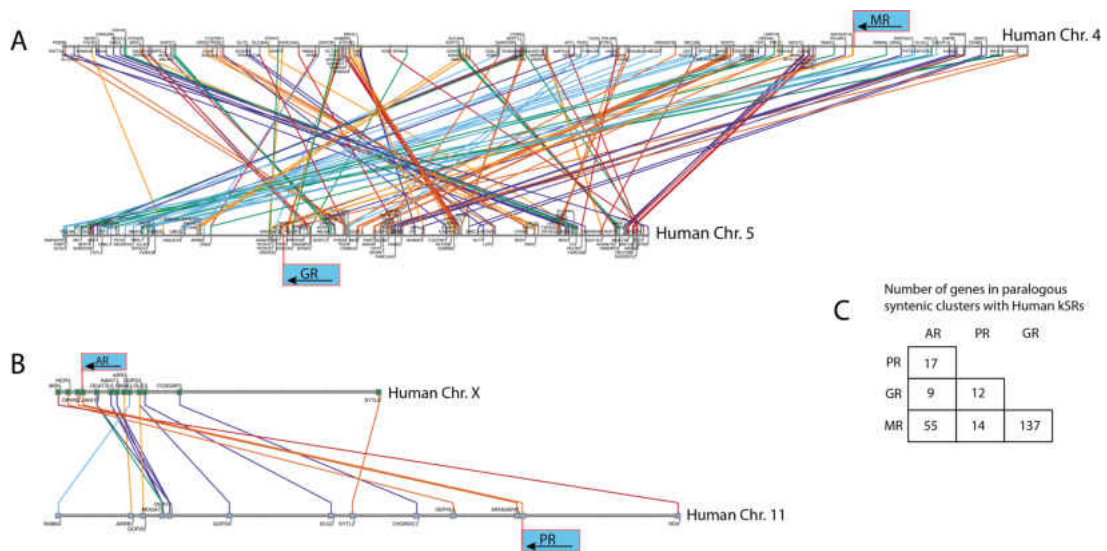
Figure S3. Vertebrate kSRs are related through duplication during the two rounds of vertebrate whole genome duplications. A. Human MR and GR syntenic genes compared. B. Human AR and PR syntenic genes compared. C. Number of genes in paralogous syntenic clusters with human kSRs.
