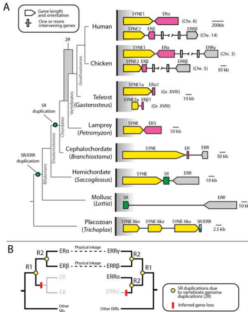
Figure 8. Relationships between SR and ERR genes are revealed by their conserved physical linkage. A. Comparative analysis of the physical linkage between basal SRs (green), ERs (pink), ERRs (grey) and an unrelated gene family (yellow) in diverse animal genomes. A single gene equally related to the SRs and ERRs (grey and green) is collinear with multiple synaptic nuclear envelope protein (SYNE) genes in the non-bilaterian placozoon, Trichoplax . In bilaterians, SRs, ERs, ERRs, and SYNEs are generally collinear, with rare intervening genes (white bar). This conserved gene organization suggests that a tandem duplication created the SR and ERR lineages at the base of Bilateria. Chromosome numbers are indicated, where known. Species relationships are shown by a cladogram, the inferred timing of gene duplications shown with green circles. B. The physical linkage of ER and ERR paralogs in vertebrates informs on their evolutionary history. The syntenic organization of ERs and ERRs in extant vertebrate genomes (Fig. S4, Appendix A) and within the ancestral chordate linkage groups (Fig. 7) suggests ERs and ERRs proliferated during 2R. One ER paralog was lost (red bar) following the first round of vertebrate genome duplication (R1), and one ERR paralogy was lost following the second round (R2).
