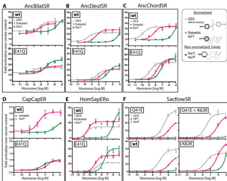
Figure 15. SacKowSR LBD recognizes aromatized steroids with a unique ligand-discriminating mechanism. Dose response curves for transcriptional activation by extant and ancestral LBDs and those mutated at critical ligand-discriminating sites. A-C. Effect of E41Q on ancestral SR function. Substitution of the ancestral E41 for the kSR-diagnostic Q41 could have drastically reduced specificity for aromatized steroids at many points in SR evolutionary history. D-E. Effect of E41Q on estrogen-specific extant receptors. The SR from the annelid Capitella capitata and the Human ER \alpha , maintain the ancestral ability to drastically reduce specificity for aromatized steroids with E41Q. F. Effect of E41Q and K82R on SacKowSR function. The aromatized ligand-specific SacKowSR was insensitive to the state at these two positions.
