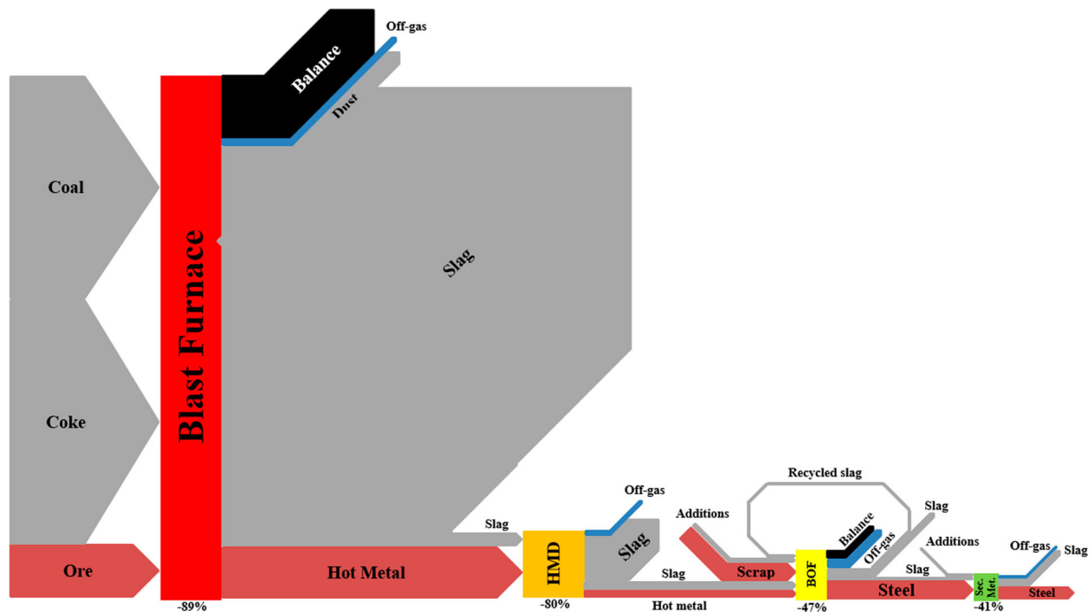
2 Sankey-type diagram of the sulphur distribution flow for a standard steel grade at Tata Steel IJmuiden in 2015. Arrows represent the amount of sulphur present in a flow, necessary for one tonne of produced steel. Below the process blocks the percentage of sulphur input that is removed in that process step is indicated
