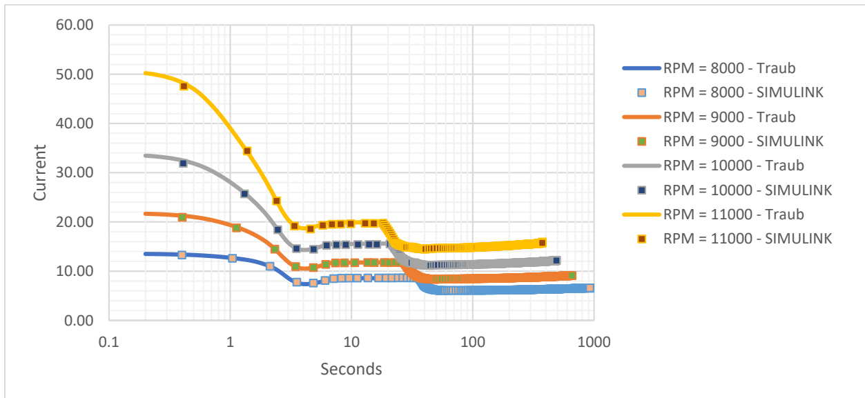
Figure 6.29 Current vs Time plot for ranging RPM values with SIMULINK simulation points
