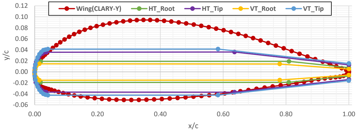
Figure 3.10 AVISTAR airfoils
