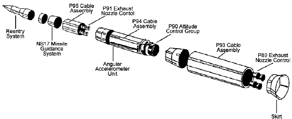
Figure 4 Minuteman II Exploded View [12]
