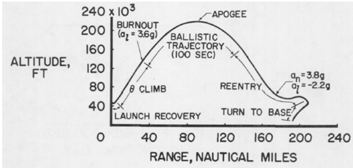
Figure 2 X-15 Altitude vs. Range Plot [11]
