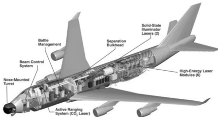
Figure 24 Boeing YAL-1 Airborne Laser [32]
