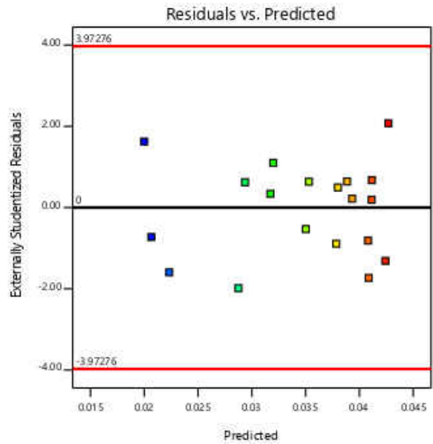
Figure 37- Residuals vs. Predicted Plots of C P for 16 in Straight Blade Aluminum Propeller
