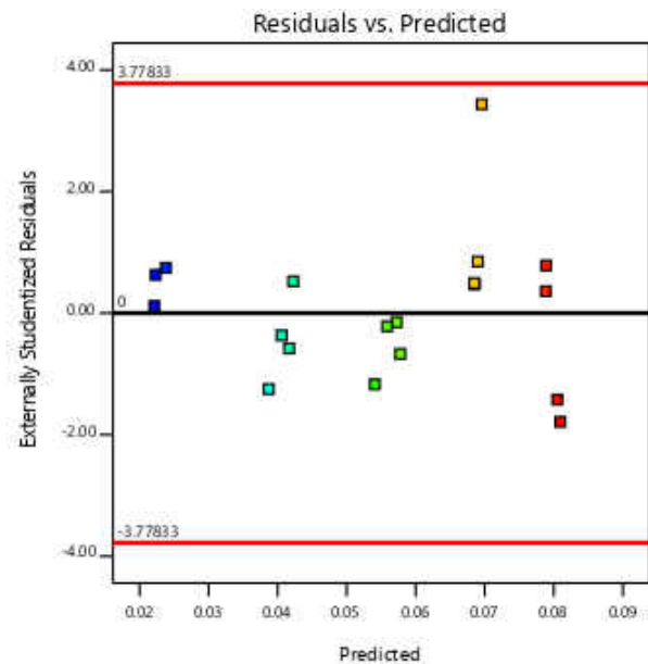
Figure 35- Residuals vs. Predicted Plots of C_T for 16 in Straight Blade Aluminum Propeller
