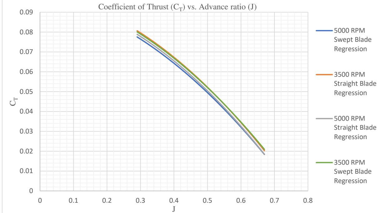
Figure 55- Coefficient of Thrust vs. Advance ratio regression model
