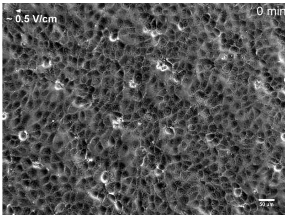
Figure 5. Phase image of 0.5 \text{ mm}^2 part of control MDCK monolayer under DCEF.
