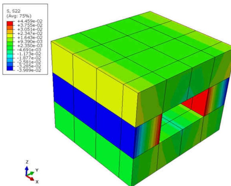
Figure 24. Stresses in the Y-direction
