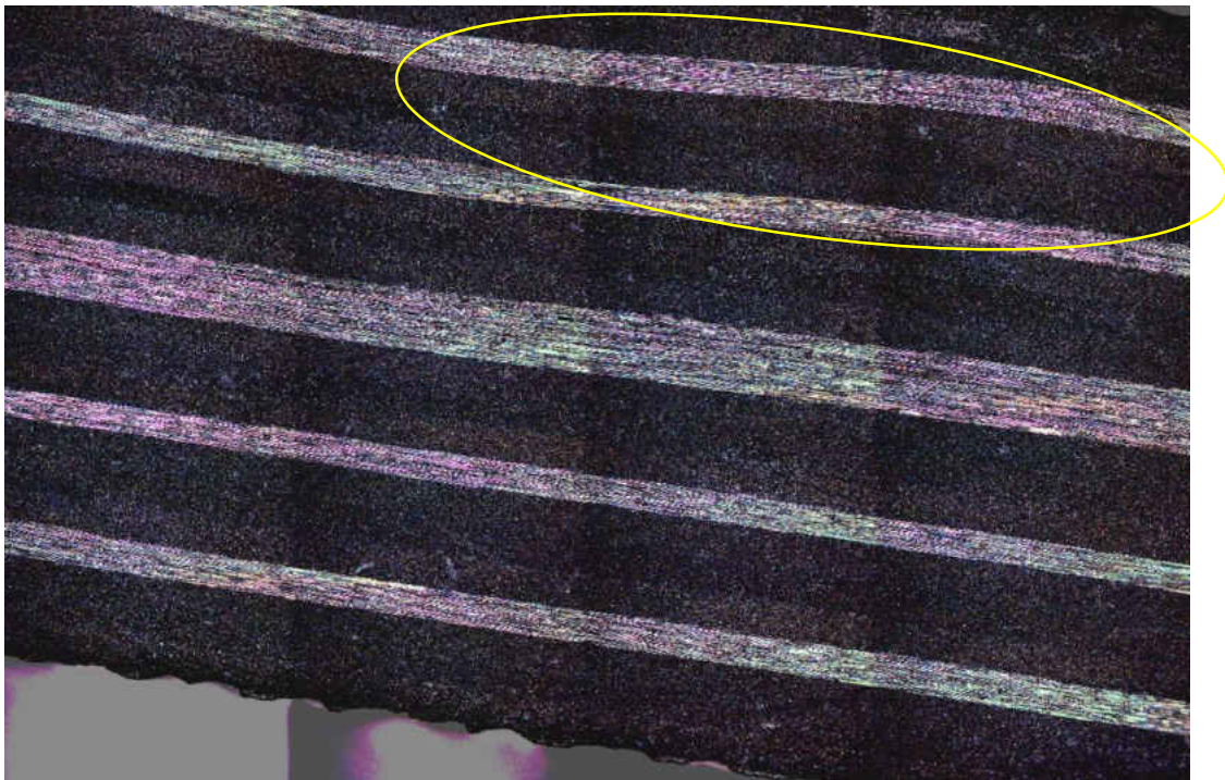
Figure 5. A micrograph of a gap in an AFP made composite which shows voids and a highlight to the 0° ply bending because of the fold.
