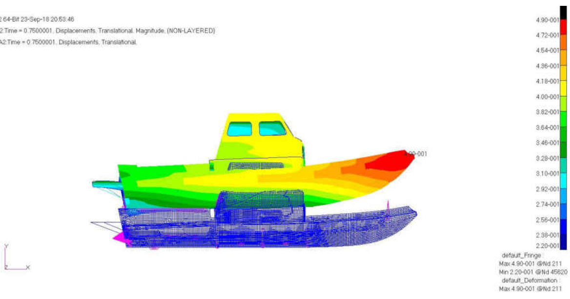
Figure C5. Side View of Deformation plot at 0.75 seconds
