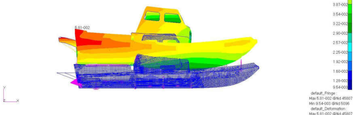
Figure C3. Side View of Deformation plot at 0.33 seconds
