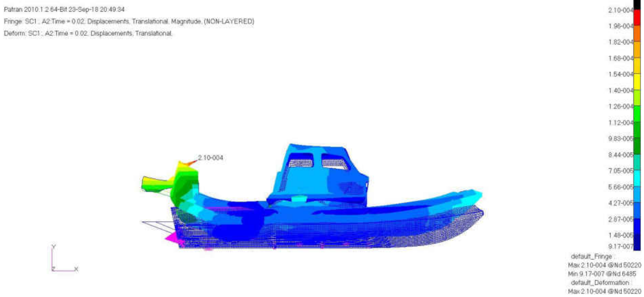
Figure C1. Side View of Deformation plot at 0.02 seconds
