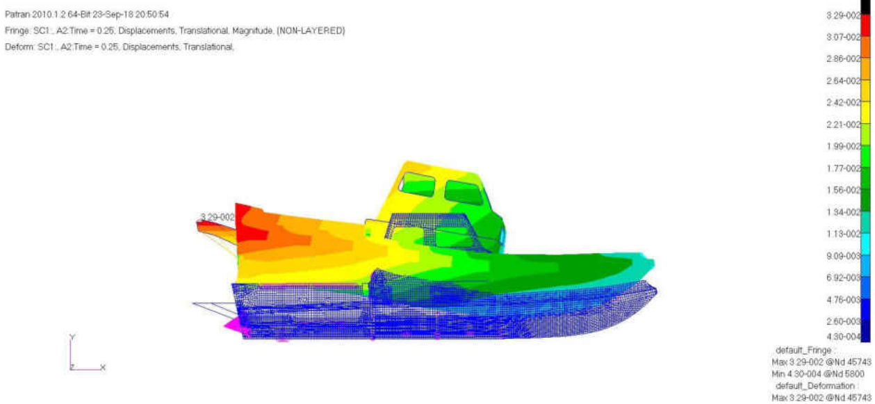
Figure C2. Side View of Deformation plot at 0.25 seconds
