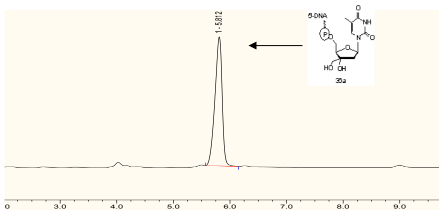
Figure 18: HPLC-of 36a
