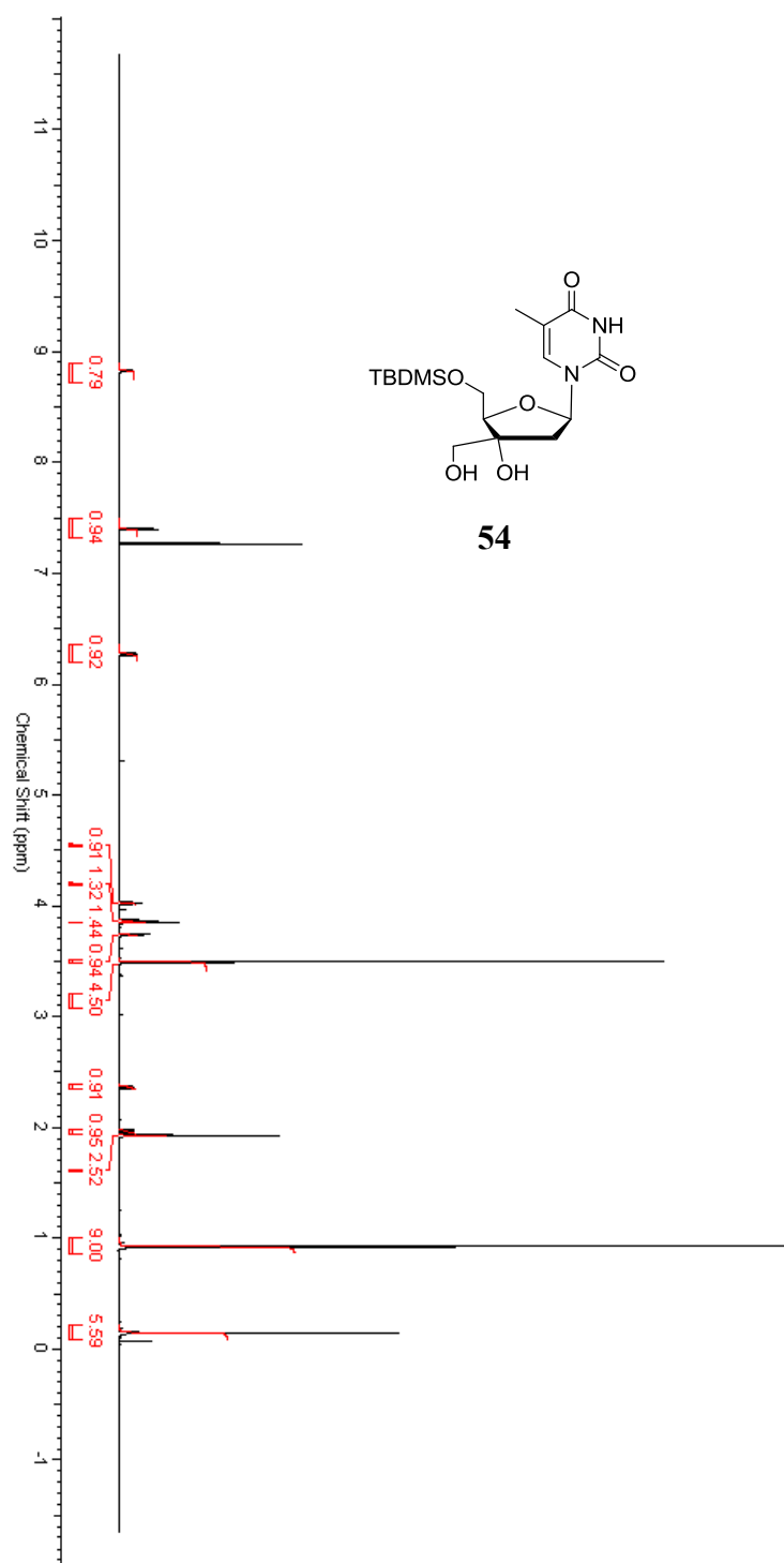
Figure 31: ^1\text{H} -NMR of compound 54
