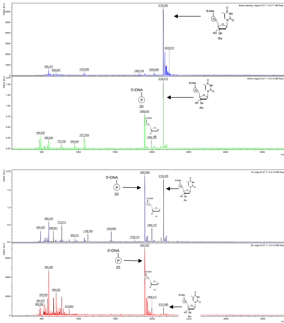
Figure 20: Reaction with NaIO 4 monitored over time
