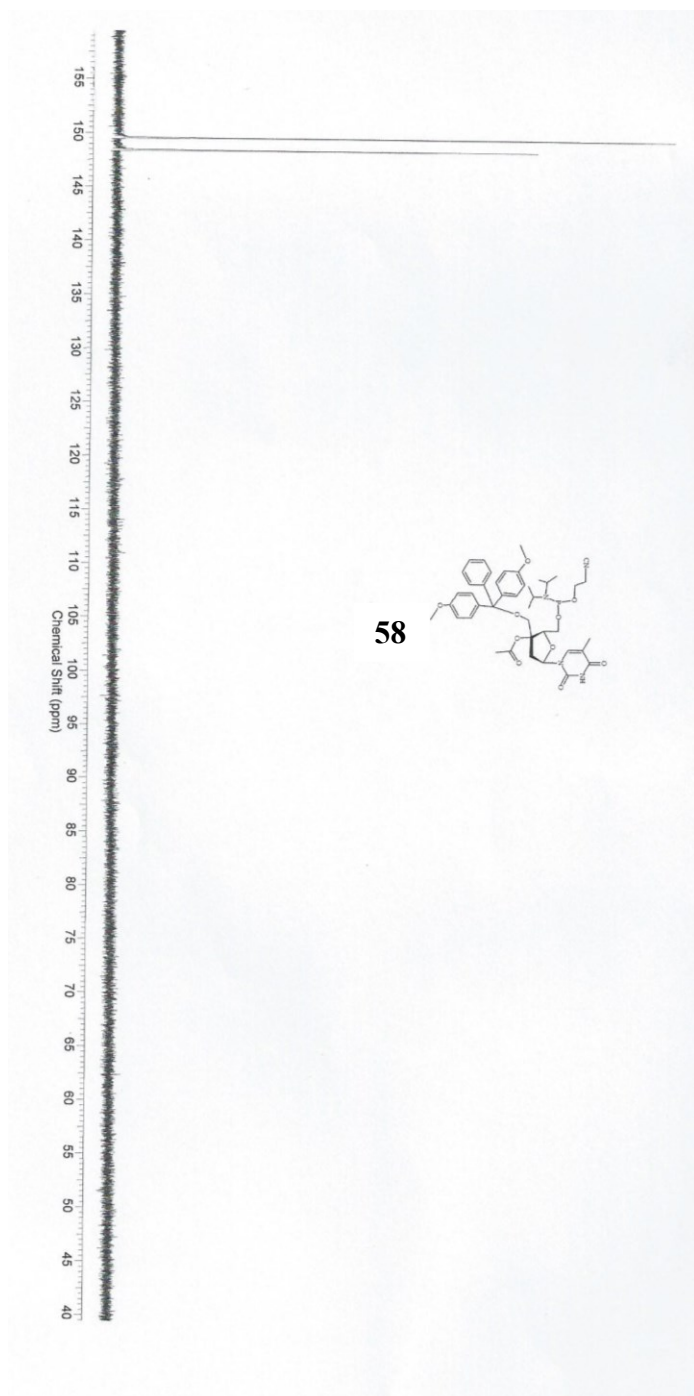
Figure 46: Phosphorus NMR of compound 58
