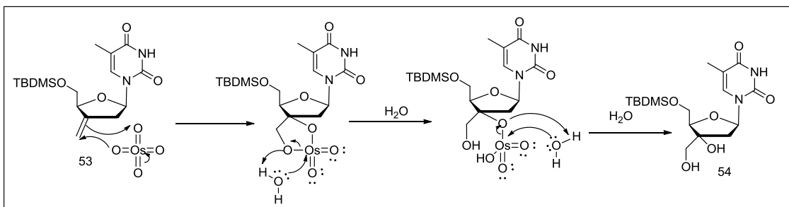
Scheme 9: Dihydroxylation with osmium tetroxide
