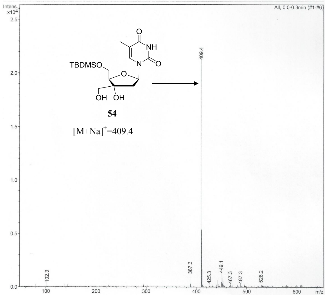
Figure 30: ESI-MS of compound 54
