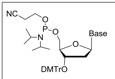
Figure 16: Nucleoside building blocks for reverse synthesis
