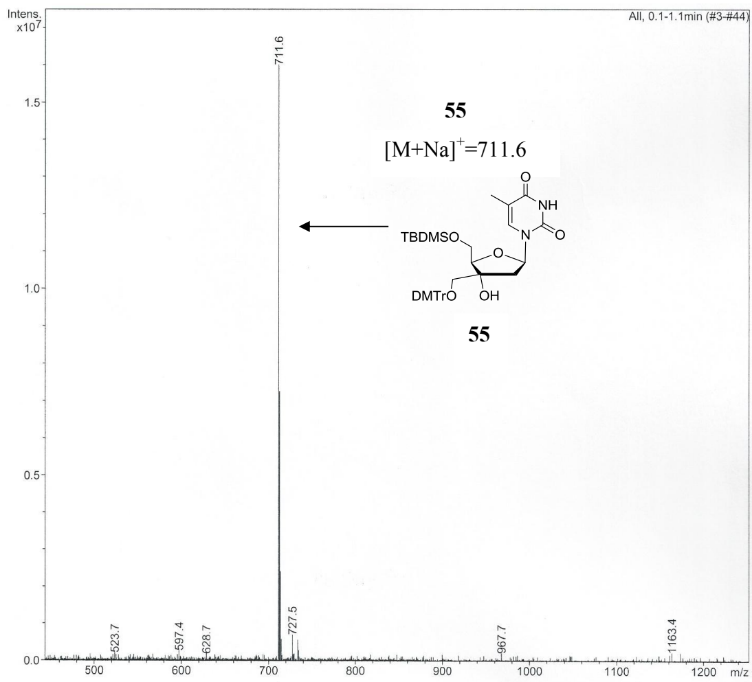
Figure 32: ESI-MS of compound 55
