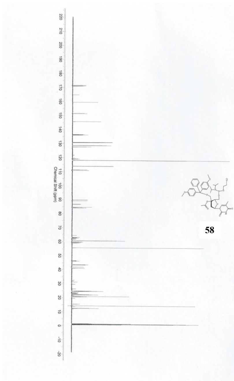
Figure 45: C-13 NMR of compound 58
