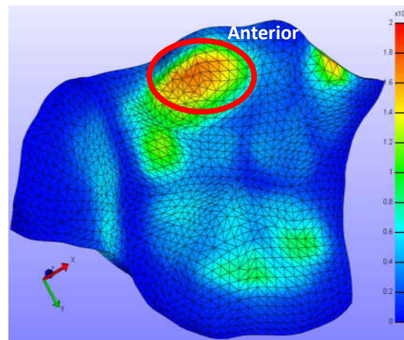
Figure 14 The inferior views of a tibia's cartilage. Ankle complex joint FE model contact stress for the neutral position with an axial nodal force 600 N. The pick stresses was ranging from 2.0541 MPa to 2.0542 MPa were in the ankle complex joint.
