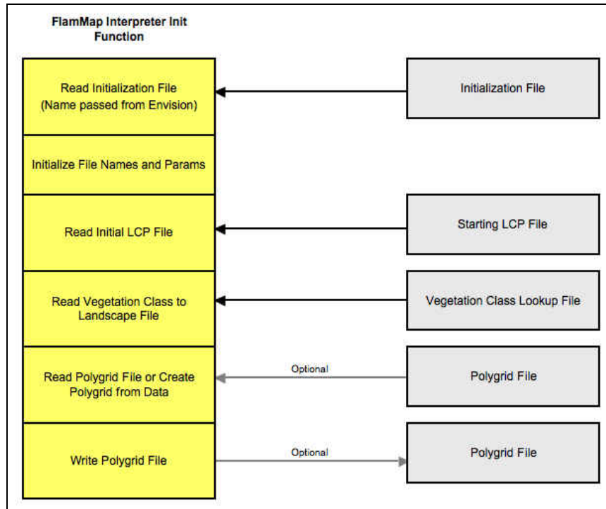
Figure 2. Functionality diagram of FlamMap Interpreter Init function.
