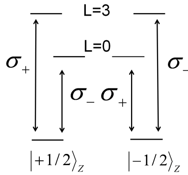
Figure 5.5 Observed D^0X transition scheme in bulk GaAs using circularly polarized light. Pulses of either polarization couple to both DBE ground states.
